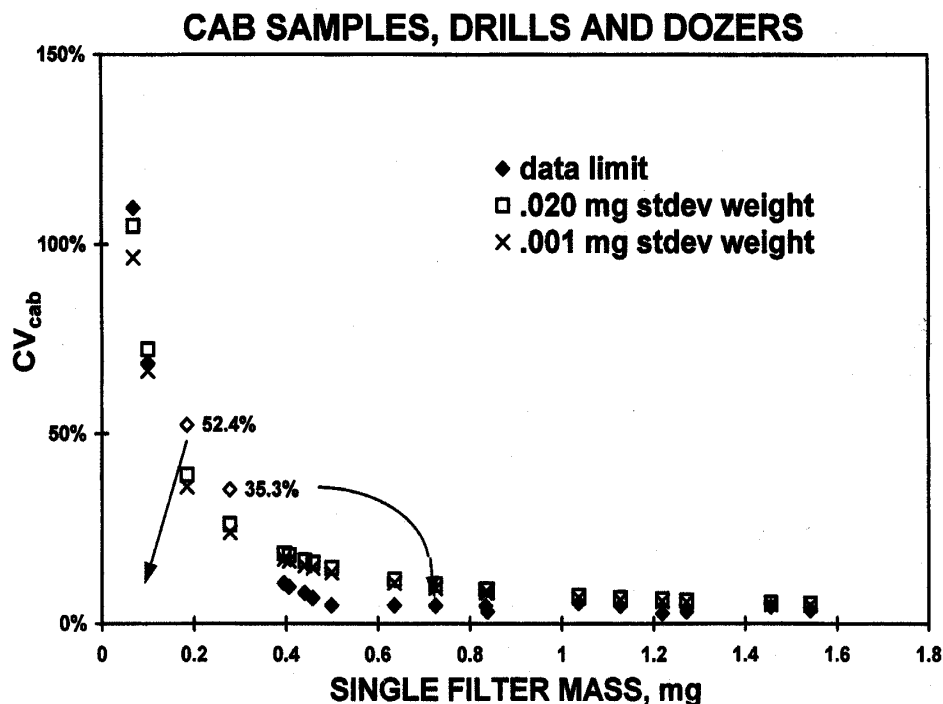
Maximum coefficient of variation ( CV ) versus single sample respirable dust mass, all sampler packages for drill and dozer cabs. Regression values shown, represented by open squares and Xs, indicate sensitivity analysis for weighing precision.
