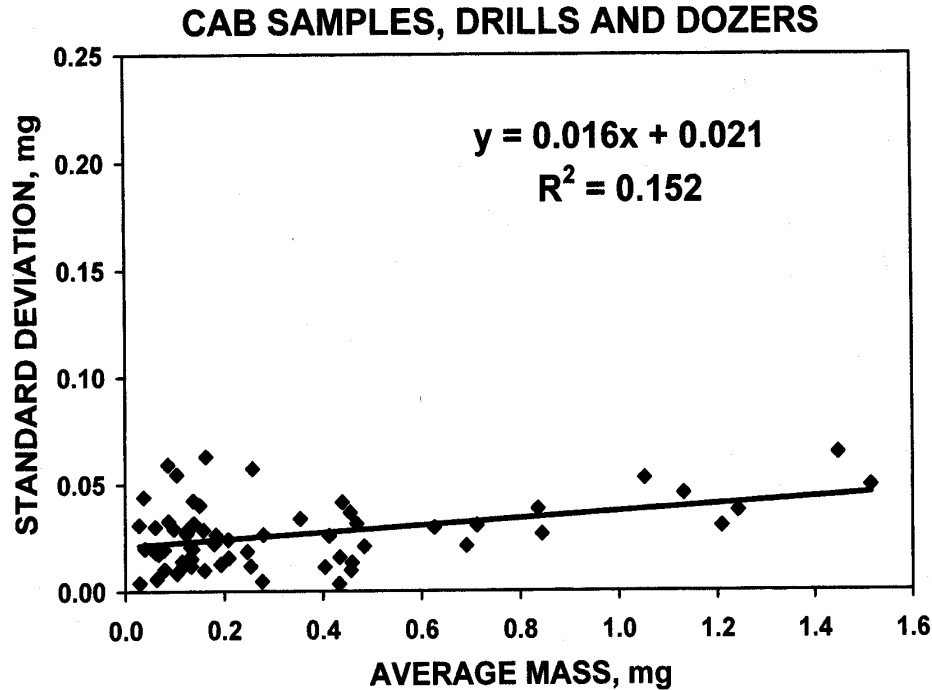
Standard deviation versus average sampler package dust mass, all sampler packages for drill and dozer cabs.
