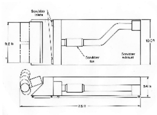
Figure 4. Scrubber location on model mining machine.
