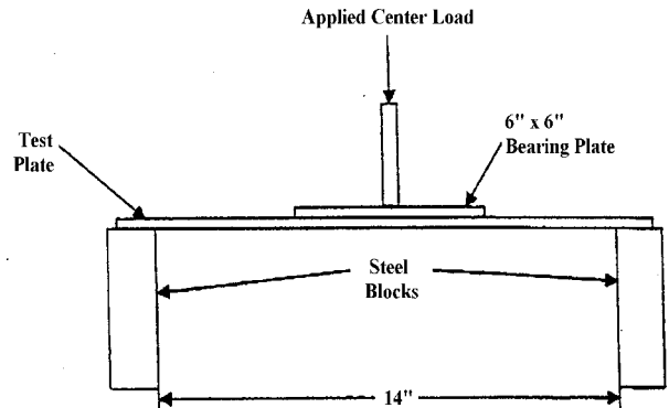
Figure 6. Test apparatus placed in Tinus Olsen machine
