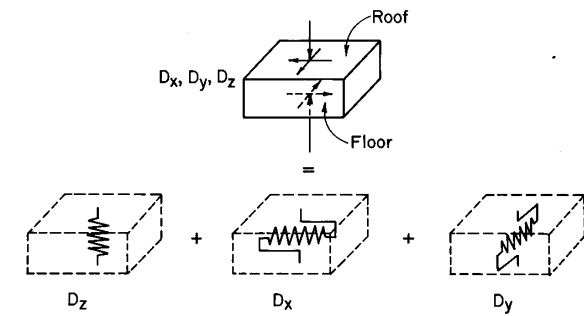
Figure 11.—Three boundary conditions applied to elemental displacement discontinuity. D_x , D_y , and D_z are elemental displacement discontinuity components.
