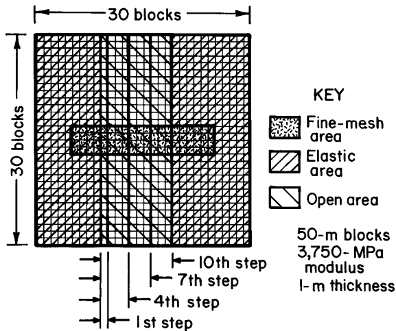
Figure 34.—MULSIM/NL grid for widening-crack problem.
