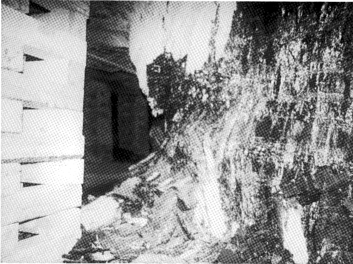
Figure 4.—Rib experiencing brittle and slabbing failure.
