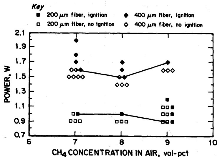
Fig. 4. Igniting powers for optical fibers tipped with PC (3 \mu\text{m} )-Krytox mixture, placed in flammable methane–air mixtures.
