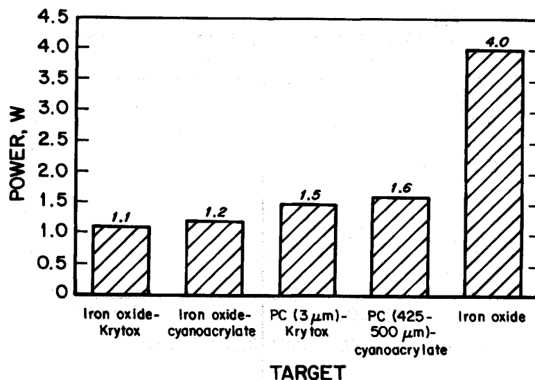
Fig. 3. Minimum igniting powers with selected targets placed on a 400 \mu\text{m} core optical fiber placed in flammable methane–air mixtures.
