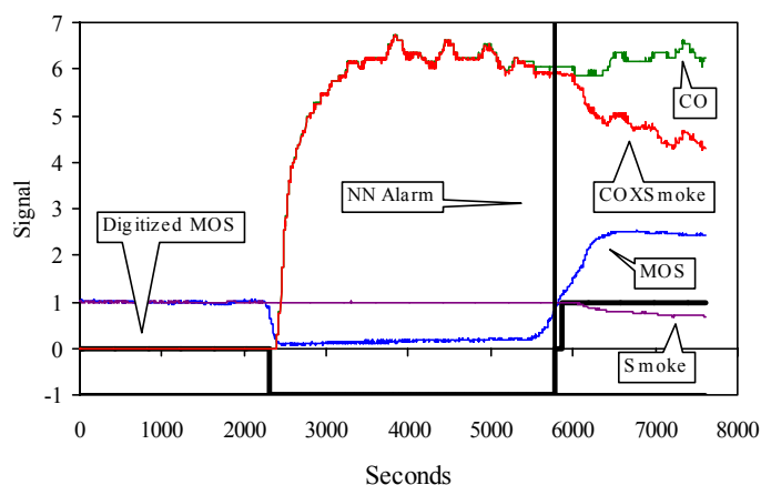
Figure 7. Inputs to the NN from station-2 data from the third belt fire with diesel exhaust.
