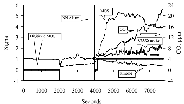
Figure 4. Inputs to the NN from station-1 data from the third coal fire with diesel exhaust.
