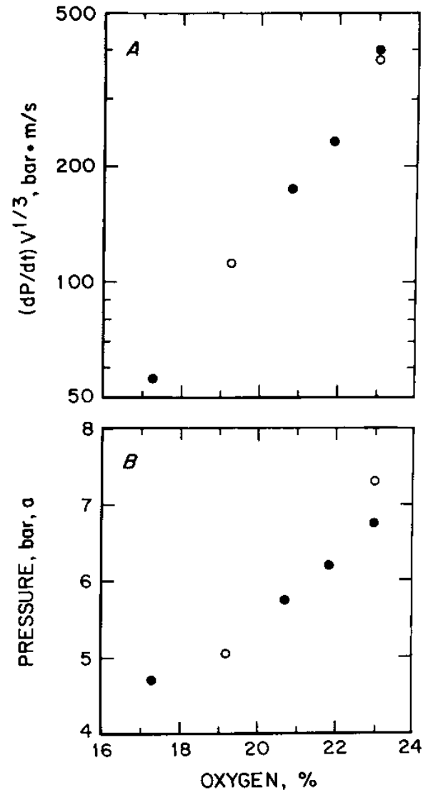
Fig. 14. Effect of oxygen concentration on explosion pressures and rates of pressure rise (data from DiPalma, 1998).
