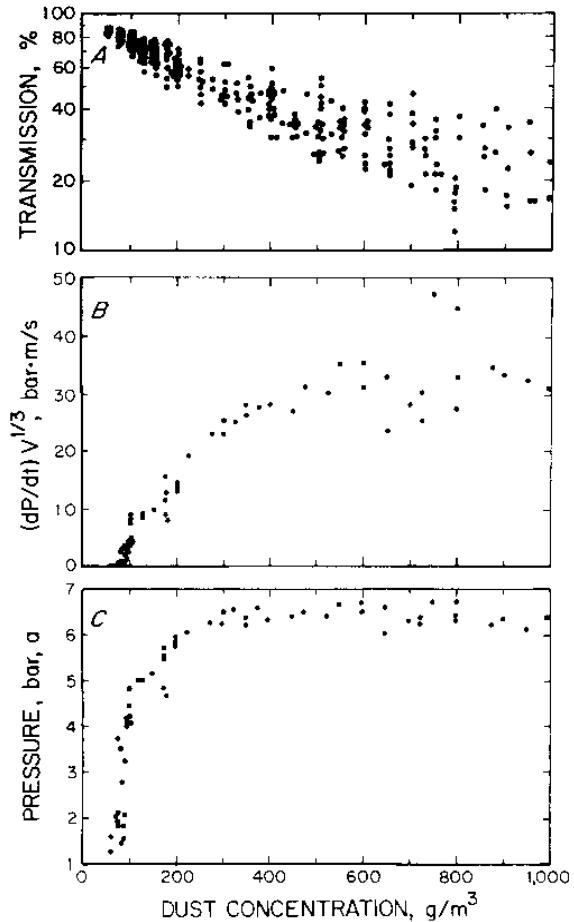
Fig. 6. Explosibility data for high volatile bituminous coal dust.
