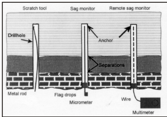
Figure 9 - Comparison of three roof monitoring techniques.
