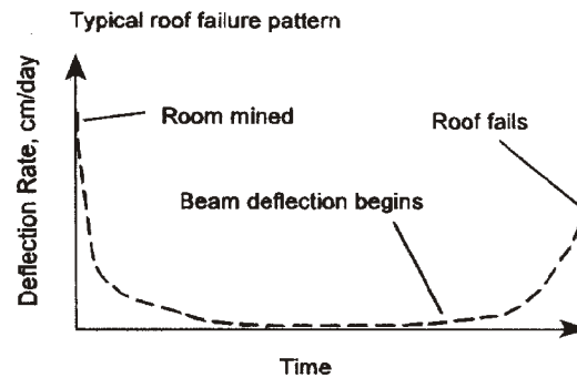
Figure 10 - Typical cycles experienced by failing stone roof beams. Note the periods of decelerating, quiet, and accelerating deflection rate.
