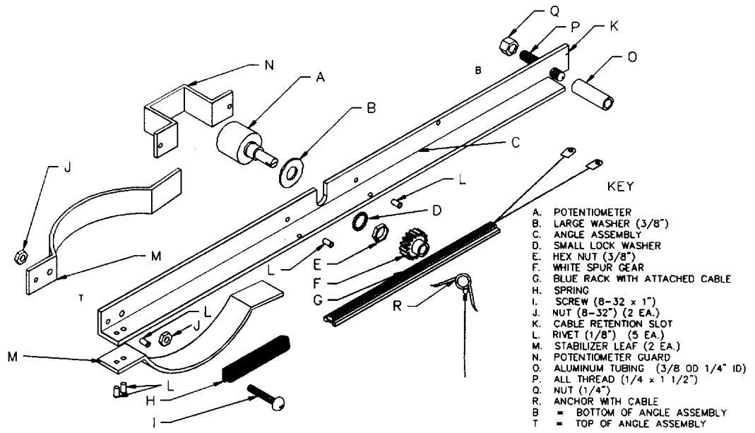
Figure 13 - Overall view of RMSS components.
