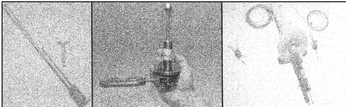
Figure 7 - Photograph of the commercially available Miners Helper, the Guardian Angel, and the RMT's Dual Height Telltale roof mechanical extensometer monitoring devices.
