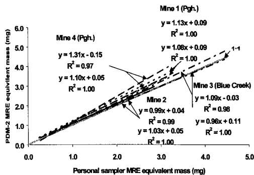
Figure 4. Individual mine response. Regression equations are for units 12 and 14 respectively.
