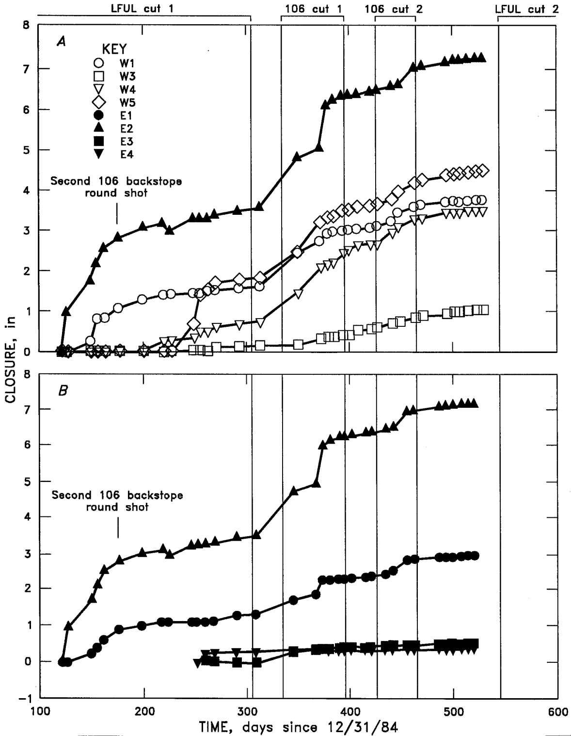
Figure 11.—Horizontal stope closure at monitoring stations in cut 1 prior to backfill placement. A, Stations west (W) of ramp; B, stations east (E) of ramp.
