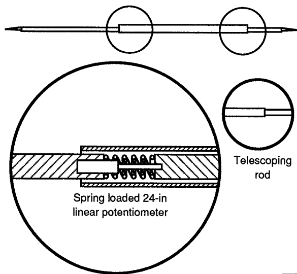
Figure 6.—Closure extensometer.
