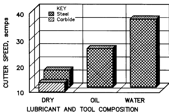
Figure 10.—Failure speed as function of lubrication environment.
