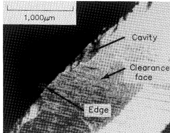
Figure 1.—Failed tungsten carbide end mill.
