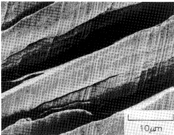
Figure 8.—Heavy striations on chip back.
