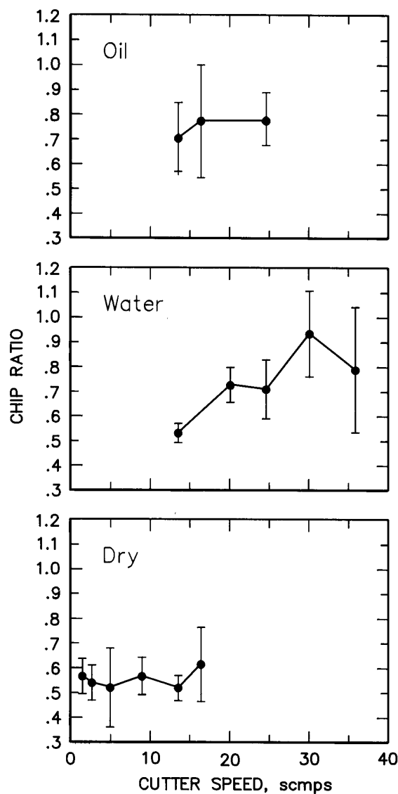
Figure 11.—Chip ratio as function of cutter speed for three lubrication environments.
