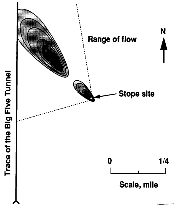
Figure 35.—Predicted flow direction of lixiviant plume (the dimensions of the plume are greatly exaggerated).
