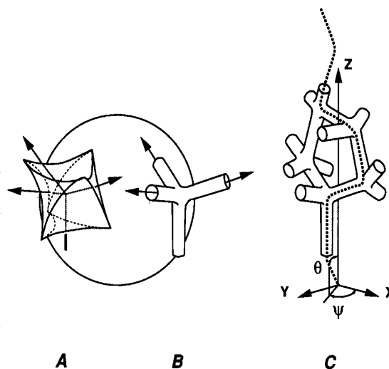
Figure 5.—Pore canal system. A, Tetrahedral pore between four spheres; B, pore schematized bifurcation; C, random path chosen by foreign particle through canal system (14).
