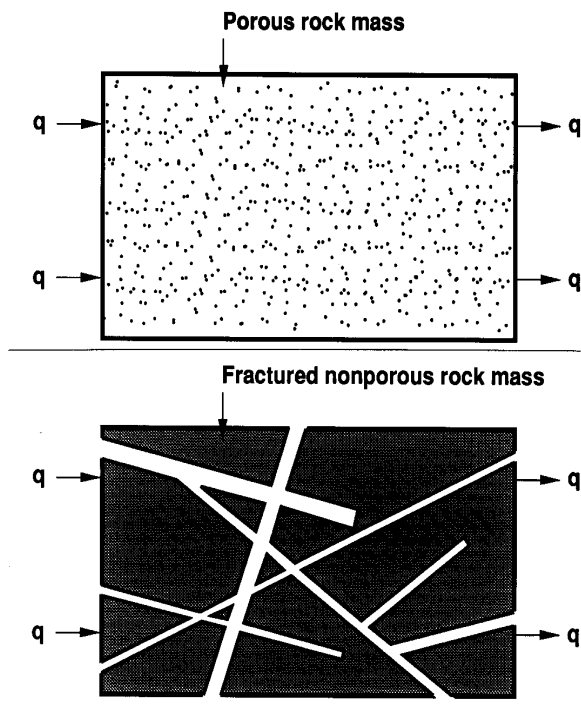
Figure 4.—Continuum (top) and noncontinuum (bottom) models, where 'q' is flow.
