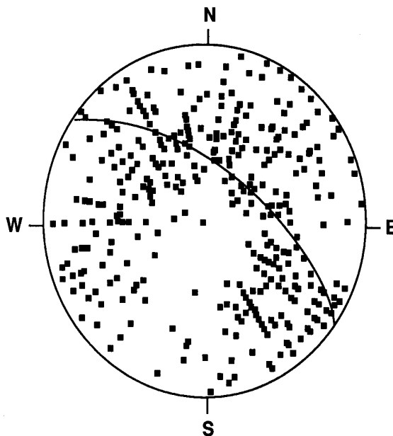
Figure 19.—Schmidt net from Edgar Mine fracture data.
