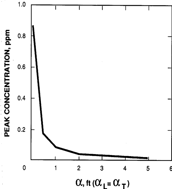
Figure 30.—Peak concentration versus dispersivity after 1 year.
