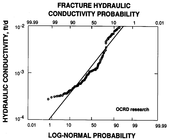
Figure 17.—Probability distribution of fracture hydraulic conductivities from research by Office of Crystalline Rock Depositories (OCRD).
