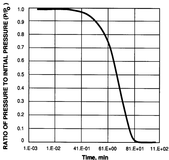
Figure 24.—Example of data to be used for curve matching.
