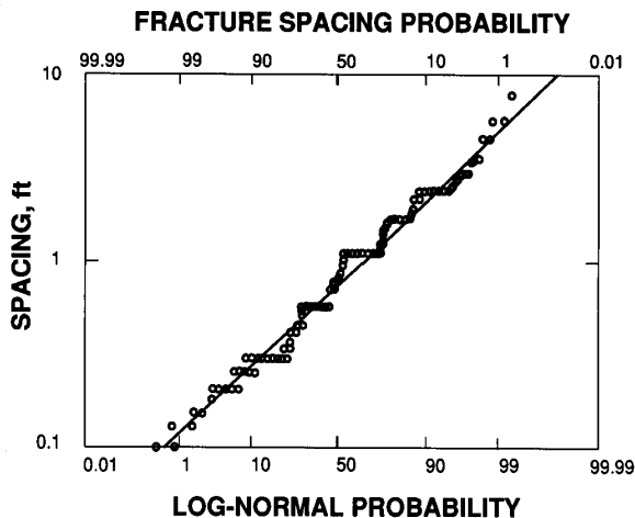
Figure 13.—Probability distribution of fracture spacing in mine.
