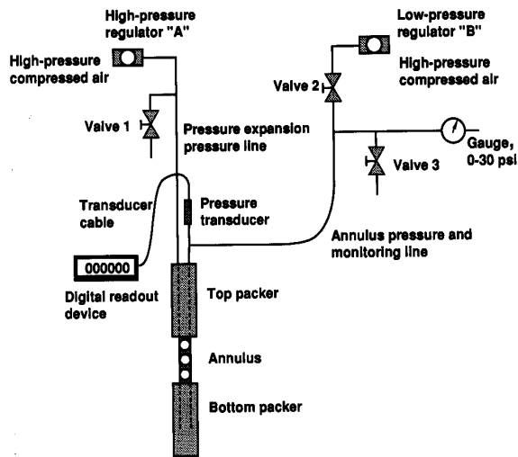
Figure 21.—Equipment setup for air packer tests.
