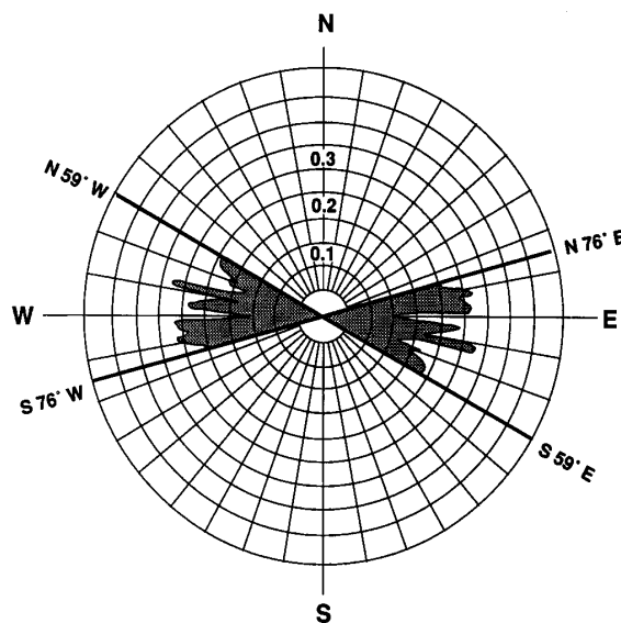
Figure 28.—Direction of ground water velocity with associated concentrations (in ppm) of plume as calculated by PLUME model.
