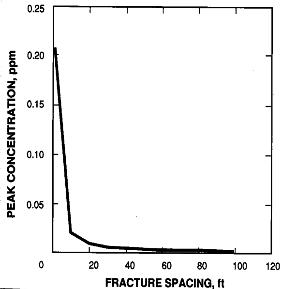
Figure 31.—Peak concentration versus fracture spacing after 1 year.
