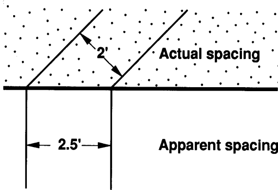
Figure 14.—Apparent spacing versus actual spacing.
