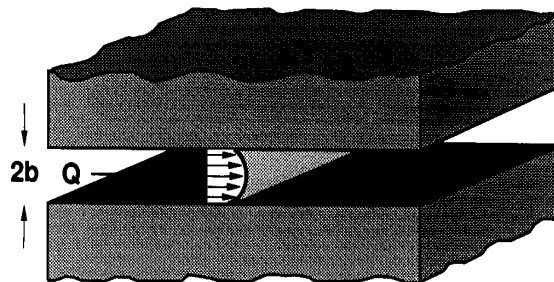
Figure 6.—Parallel plates illustrating Cubic law. Q = volume flow rate; 2b = aperture of fracture.
