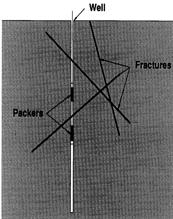
Figure 27.—Avenues of air loss during air packer tests.
