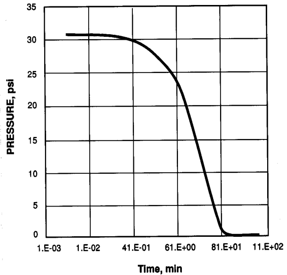
Figure 23.—Example of raw data from air packer test.
