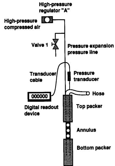
Figure 22.—Equipment setup for water packer tests.
