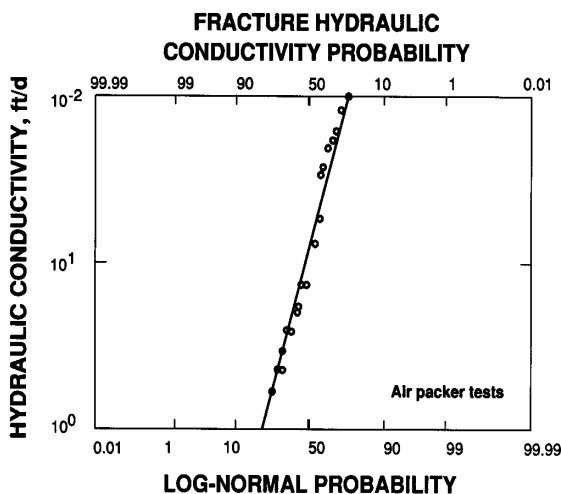
Figure 18.—Probability distribution of fracture hydraulic conductivities from air packer tests.
