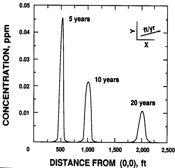
Figure 29.—Concentration versus distance with time as third variable.
