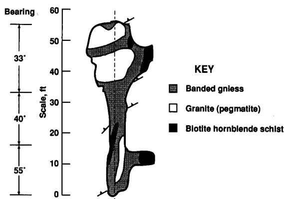
Figure 7.—Geology of experimental stope site.
