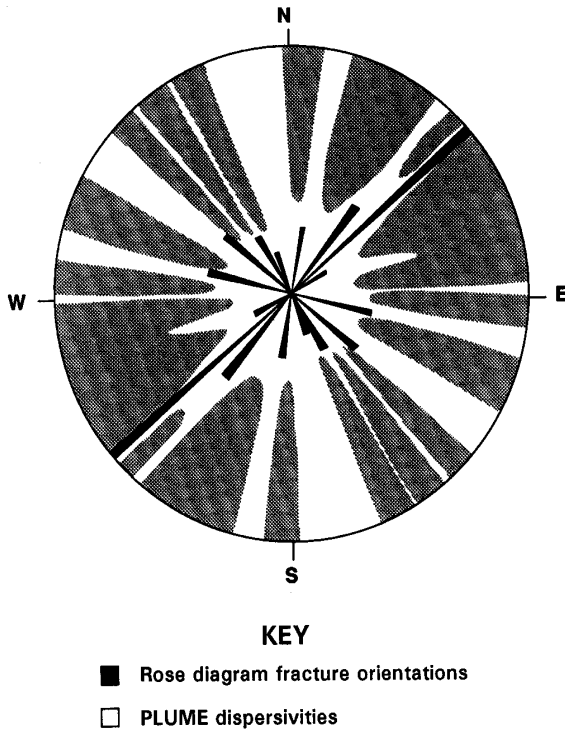
Figure 20.—PLUME model dispersivities versus rose diagram for slope site fracture dip orientations.
