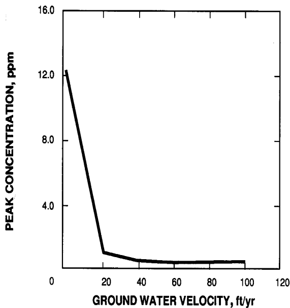
Figure 32.—Peak concentration versus ground water velocity after 1 year.
