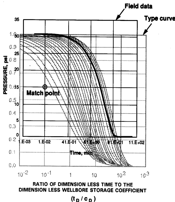
Figure 26.—Curve matching example.
