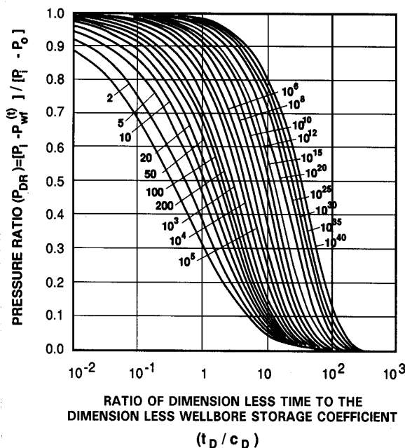
Figure 25.—Type curves for drill stem tests or slug tests (34).
