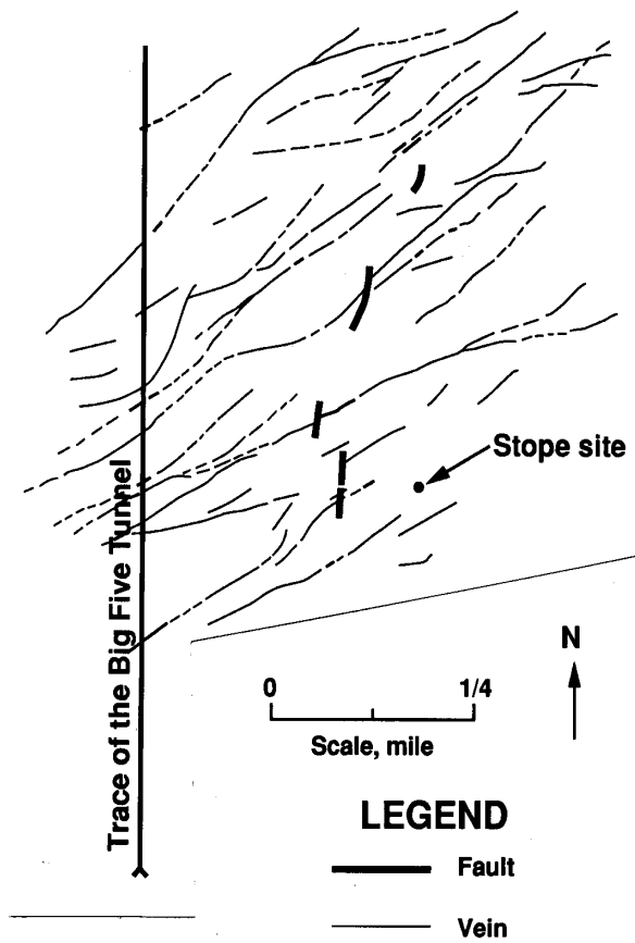
Figure 34.—Map of Idaho Springs area showing Big Five Tunnel, fault, and vein locations.
