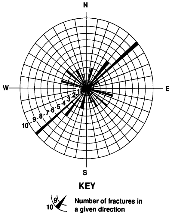
Figure 10.—Rose diagram of core fracture dip orientations from test wells.
