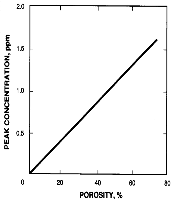
Figure 33.—Peak concentration versus porosity after 1 year.
