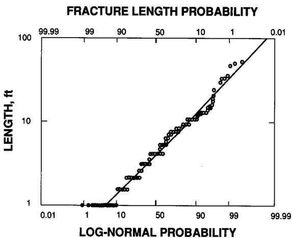
Figure 15.—Probability distribution of fracture trace length.
