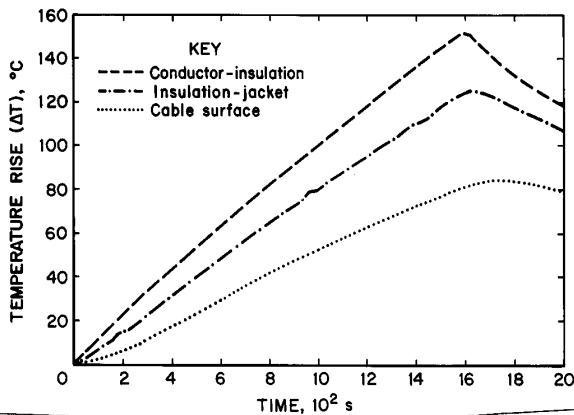
Figure 13.—Light (200% rating) overload on #2/0 AWG, 3/C, round, G-GC cable.
