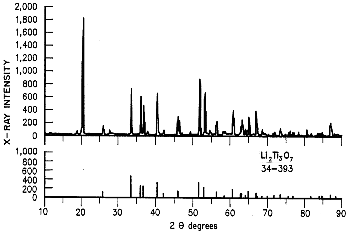
Figure 2.—X-ray diffraction patterns, orthorhombic \text{Li}_2\text{Ti}_3\text{O}_7 . Top, Graph is the actual pattern, and the bottom graph is the reference pattern.
