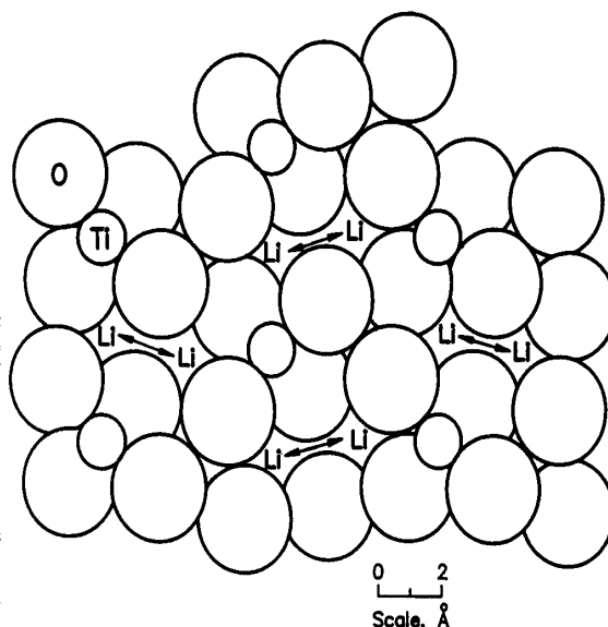
Figure 5.—Orthorhombic phase viewed along the [001] direction with the oxygen and titanium ions drawn to scale. Lithium atoms are not shown, but their positions in the tunnels are indicated with "Li" (8).
