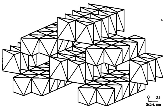
Figure 4.—Orthorhombic phase showing tunnels and arrangement of the octahedra (8).
