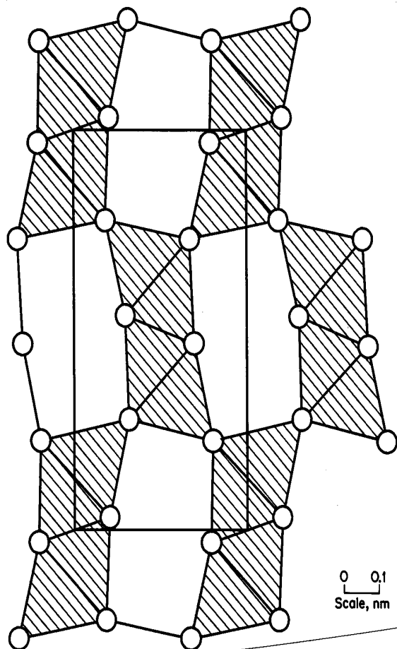
Figure 3.—Cross section of orthorhombic unit cell (12).
