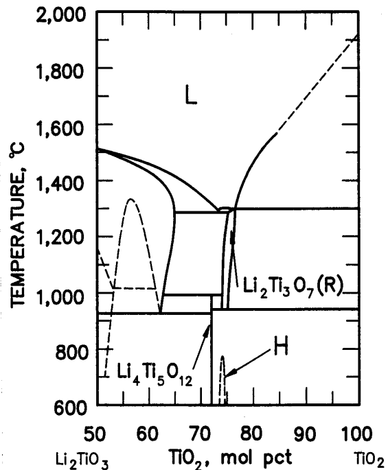
Figure 1.—Pseudobinary phase of \text{Li}_2\text{O-TiO}_2 from 50 to 100 mol pct \text{TiO}_2 (11). L = liquid; R = orthorhombic phase; H = hexagonal phase.
