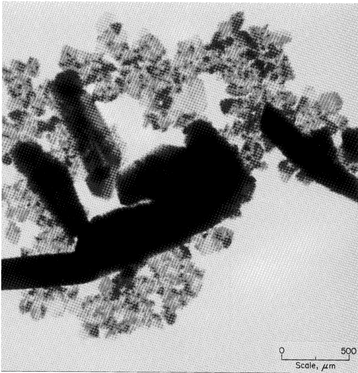
Figure 8.—TEM micrograph, orthorhombic and hexagonal phase. The octahedra are clearly visible. The dark shapes are possible hexagonal crystals viewed along the "c" direction.
