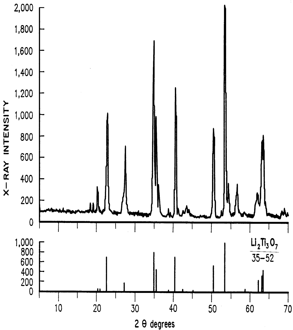
Figure 6.—X-ray diffraction patterns, hexagonal \text{Li}_2\text{Ti}_3\text{O}_7 . Top, Graph is the actual pattern, and the bottom graph is the reference pattern.
