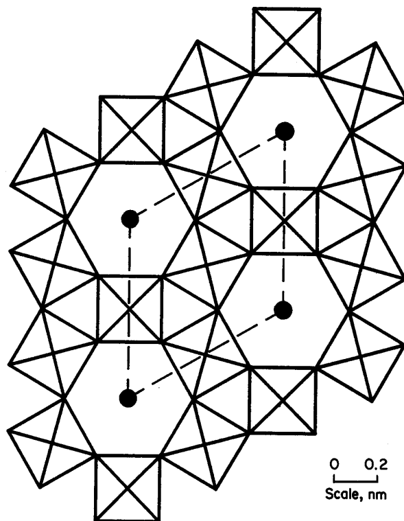
Figure 7.—Hexagonal unit cell crystal structure (8).
