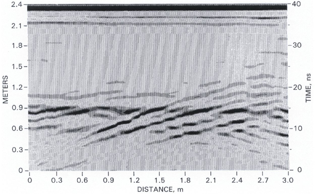
Figure 9.—GPR record at hole No. 3 at Lake Lynn.
