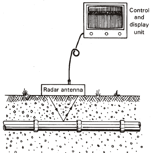
Figure 1.—GPR ray paths penetrating the ground and producing a wiggly trace on the control panel.
