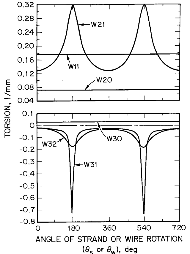
Figure 16 Torsion of IWRC and S3 wires.
