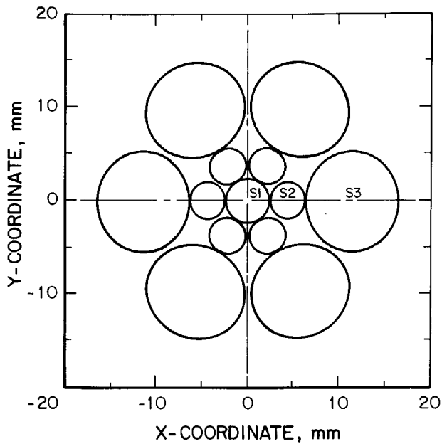
Figure 6.C Strand arrangement of 33-mm 6x19 Seale, IWRC, right regular lay wire rope.
