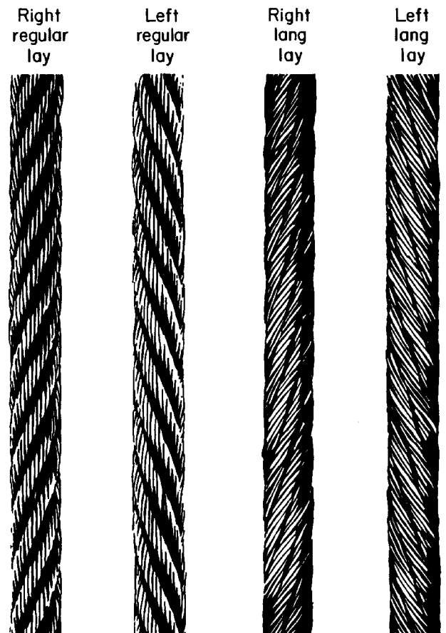
Figure 2.C Comparison of typical wire rope lays.
