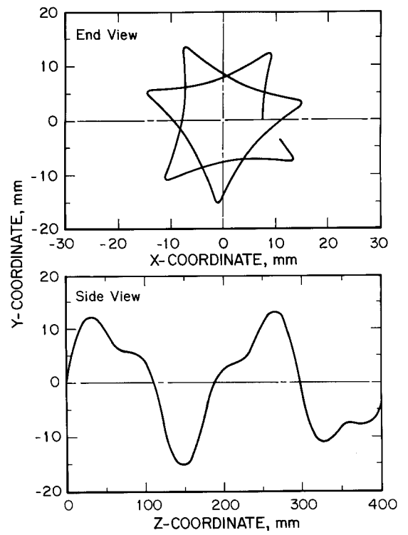
Figure 13 Path of double helical wire W32.
