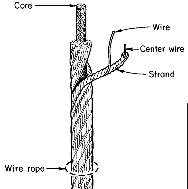
Figure 1.C Structural elements in a typical wire rope.
