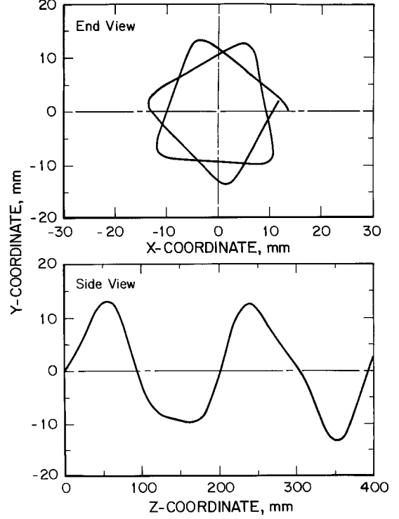
Figure 12 Path of double helical wire W31.
