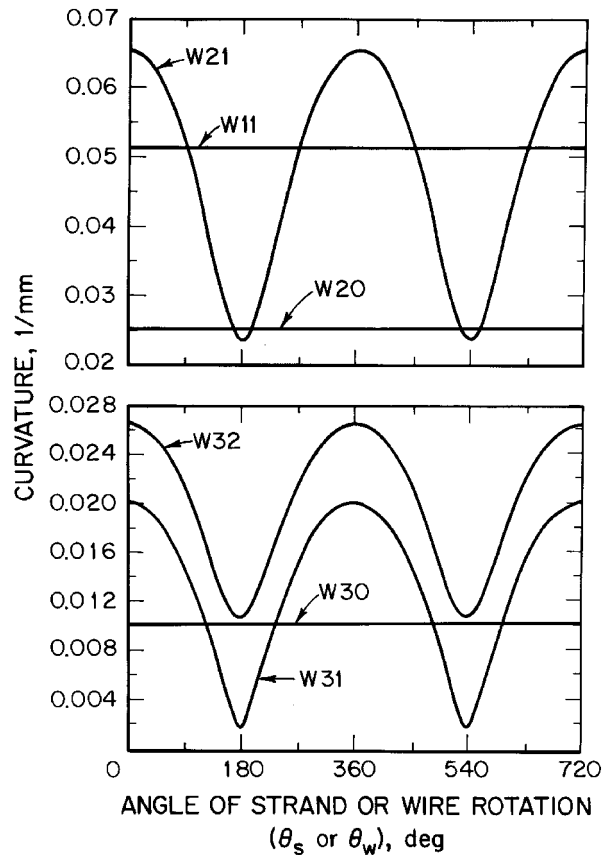
Figure 15: Curvature of IWRC and S3 wires.
