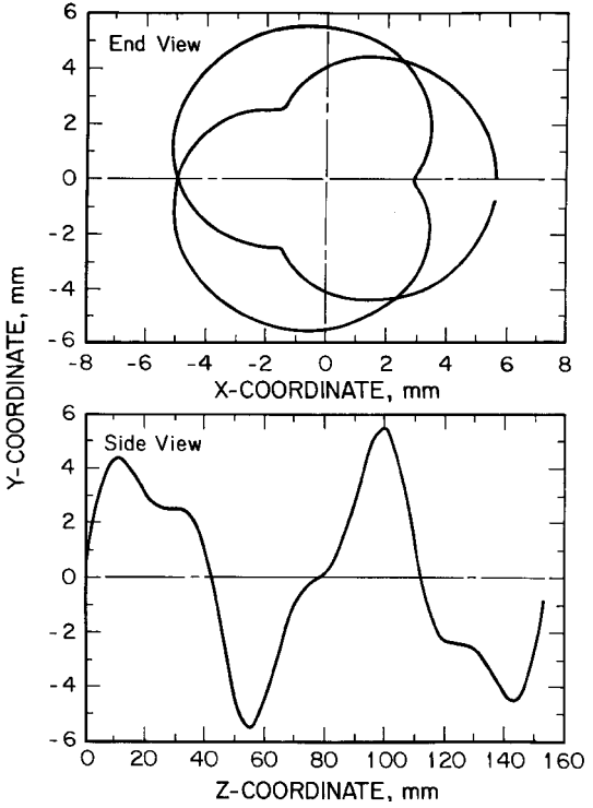
Figure 11 Path of double helical wire W21.
