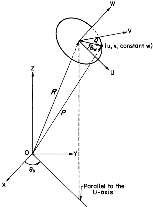
Figure 5. Coordinate system for double helix.
