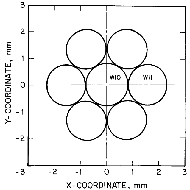
Figure 7.C Cross section of IWRC strand S1.
