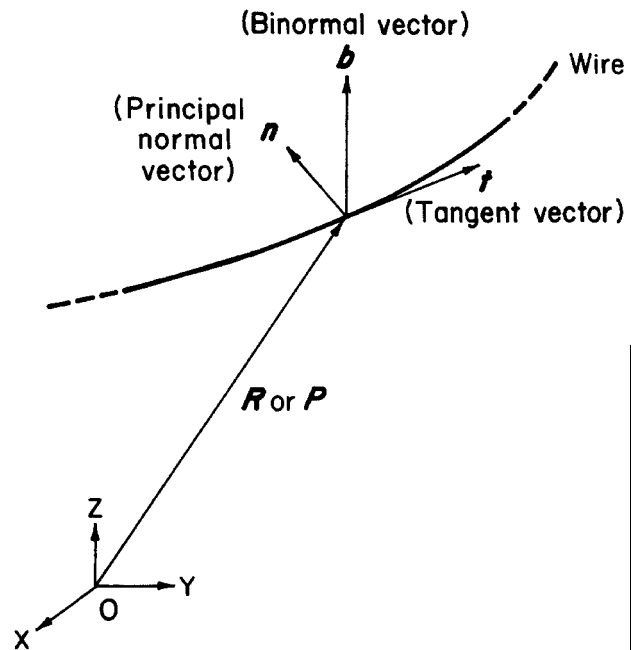
Figure 14 The moving trihedral.
