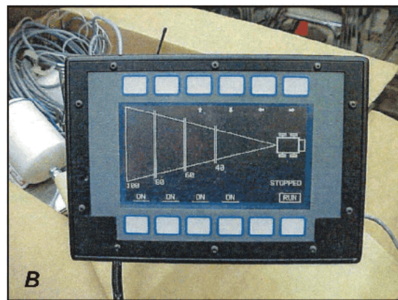
Figure 33.—Prototype radar system. A, Antenna and electronics enclosure; B, operator display showing range gates.
