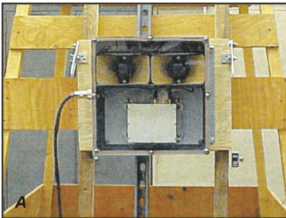
Figure 33.—Prototype radar system. A, Antenna and electronics enclosure; B, operator display showing range gates.
