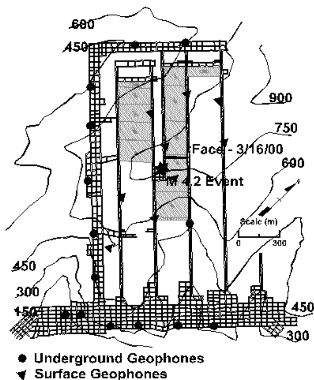
Figure 2. Plan view showing mine layout, overburden, geophone arrays, and the location of the M_L 4.2 event
