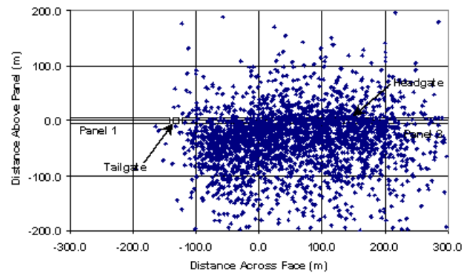
Figure 9. Vertical view parallel to the longwall face showing the normalized event locations for the last quarter of Panel 2.
