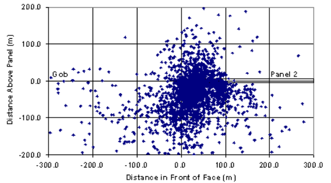
Figure 7. Vertical view parallel to face advance showing the normalized event locations for the last quarter of Panel 2.
