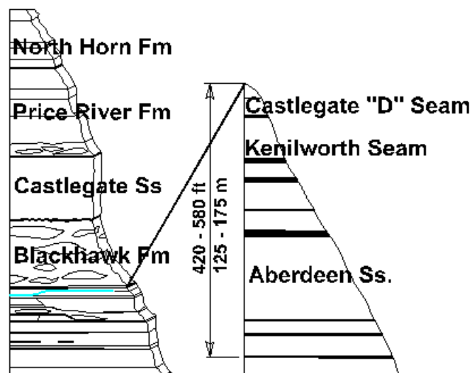
Figure 1. Generalized stratigraphy.
