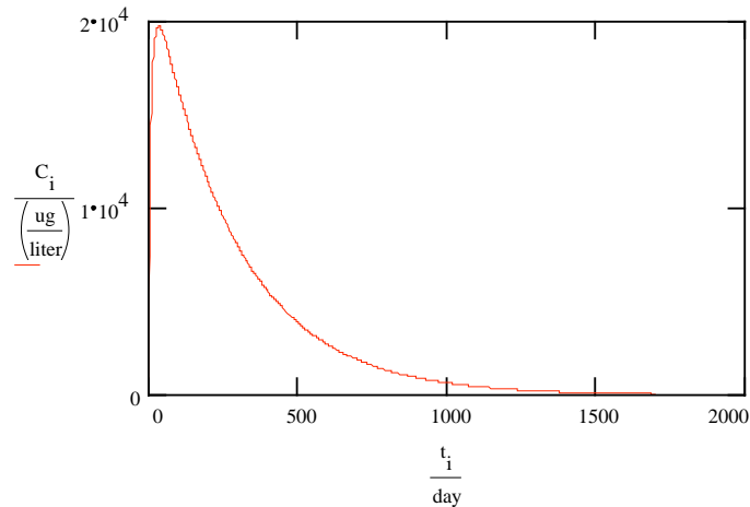
Concentration versus time at a point 10 m downgradient of the source
