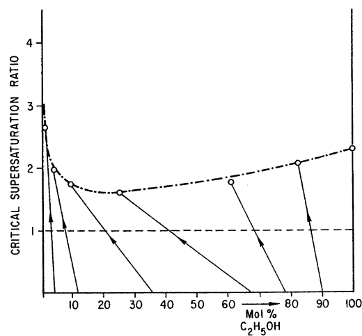
FIGURE 7. Critical supersaturation ratios for homogeneous nucleation of liquid from water-ethanol vapors. (After Flood, 1934)
