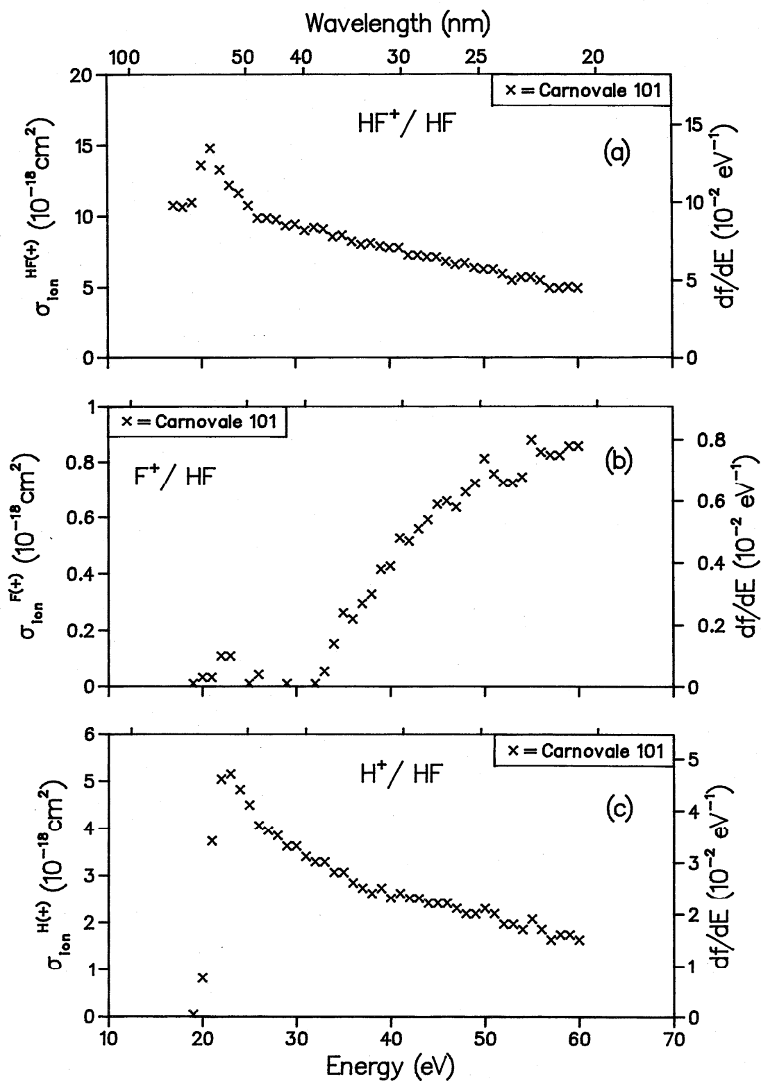
FIG. 66. Partial ionic photofragmentation cross sections for HF; (a) product ion = \text{HF}^+ , (b) product ion = \text{F}^+ , (c) product ion = \text{H}^+ .
