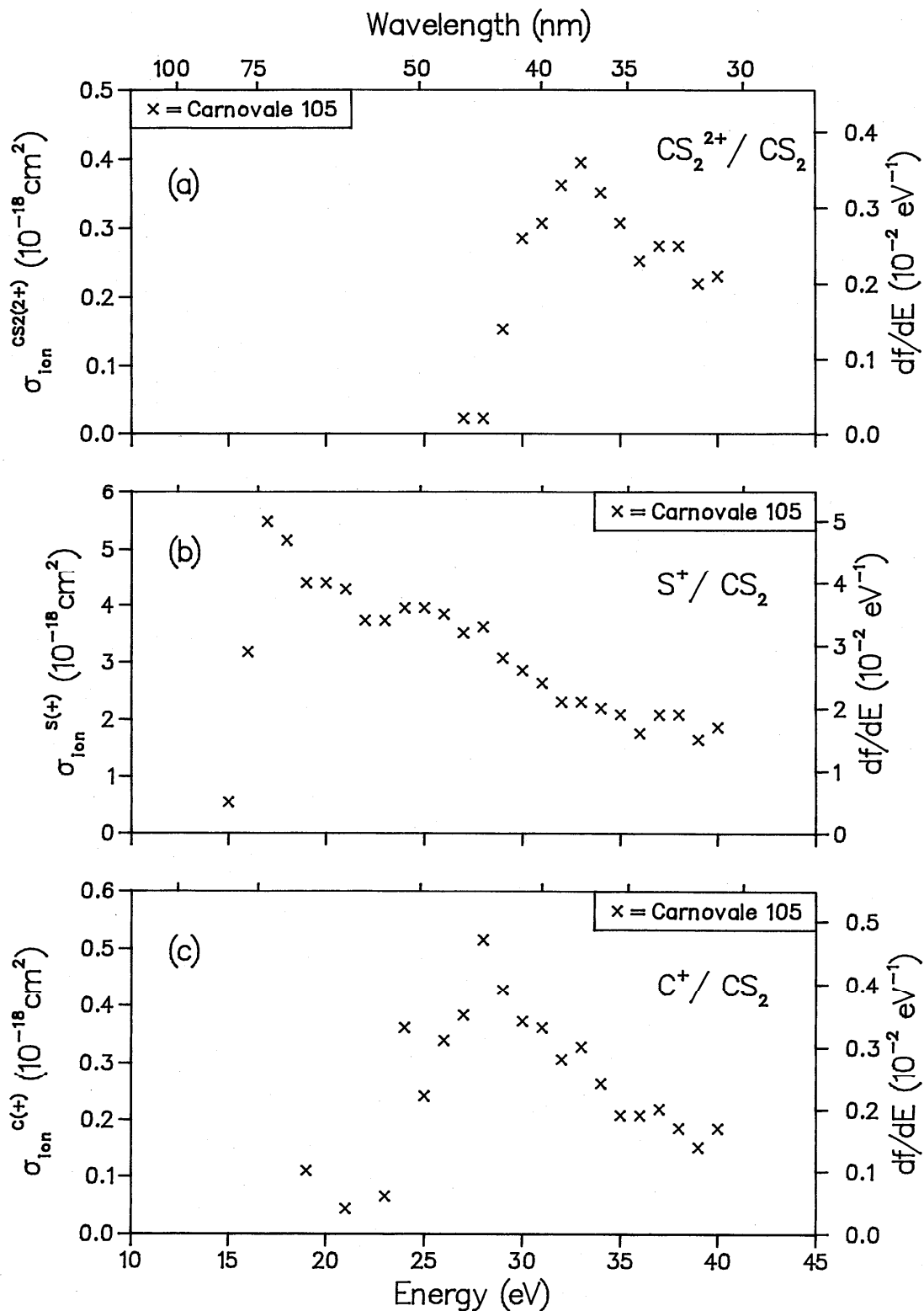
FIG. 86. Partial ionic photofragmentation cross sections for \text{CS}_2 ; (a) product ion = \text{CS}_2^{2+} , (b) product ion = \text{S}^+ , (c) product ion = \text{C}^+ .
