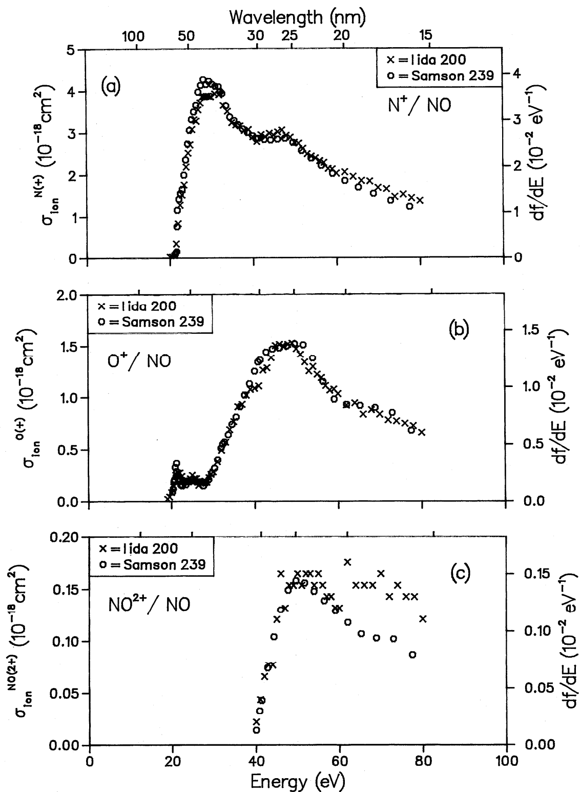
FIG. 36. Partial ionic photofragmentation cross sections for NO; (a) product ion = \text{N}^+ , (b) product ion = \text{O}^+ , (c) product ion = \text{NO}^{2+} .
