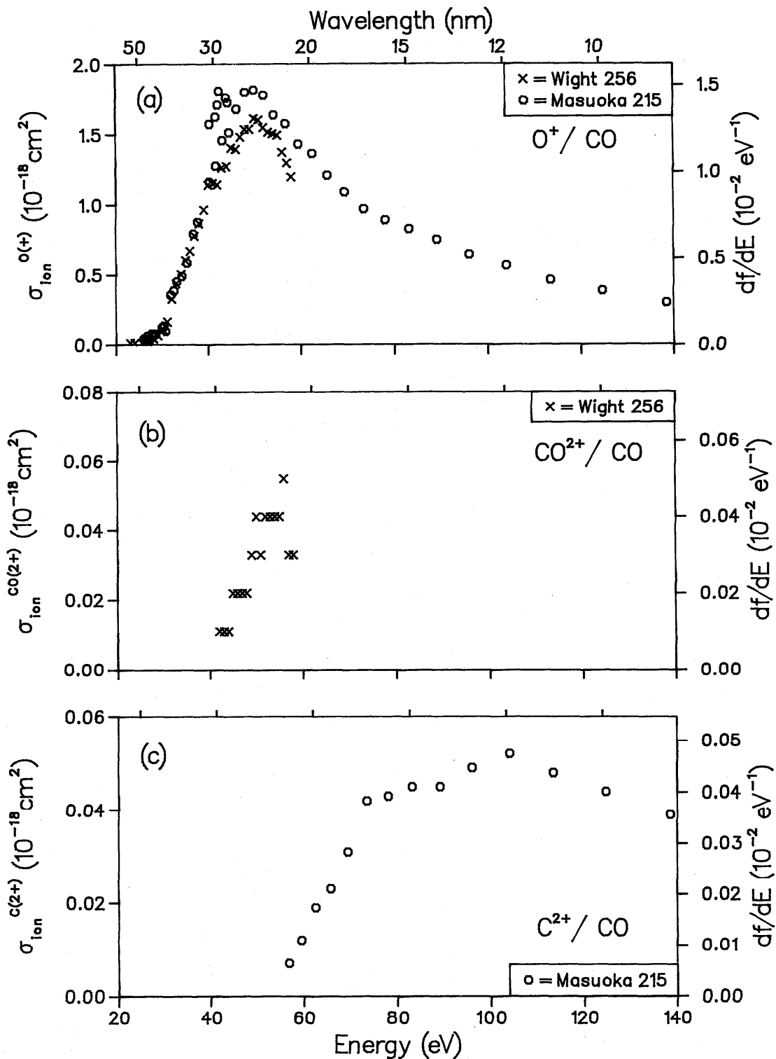
FIG. 29. Partial ionic photofragmentation cross sections for CO; (a) product ion = O + , (b) product ion = CO 2+ , (c) product ion = C 2+ .
