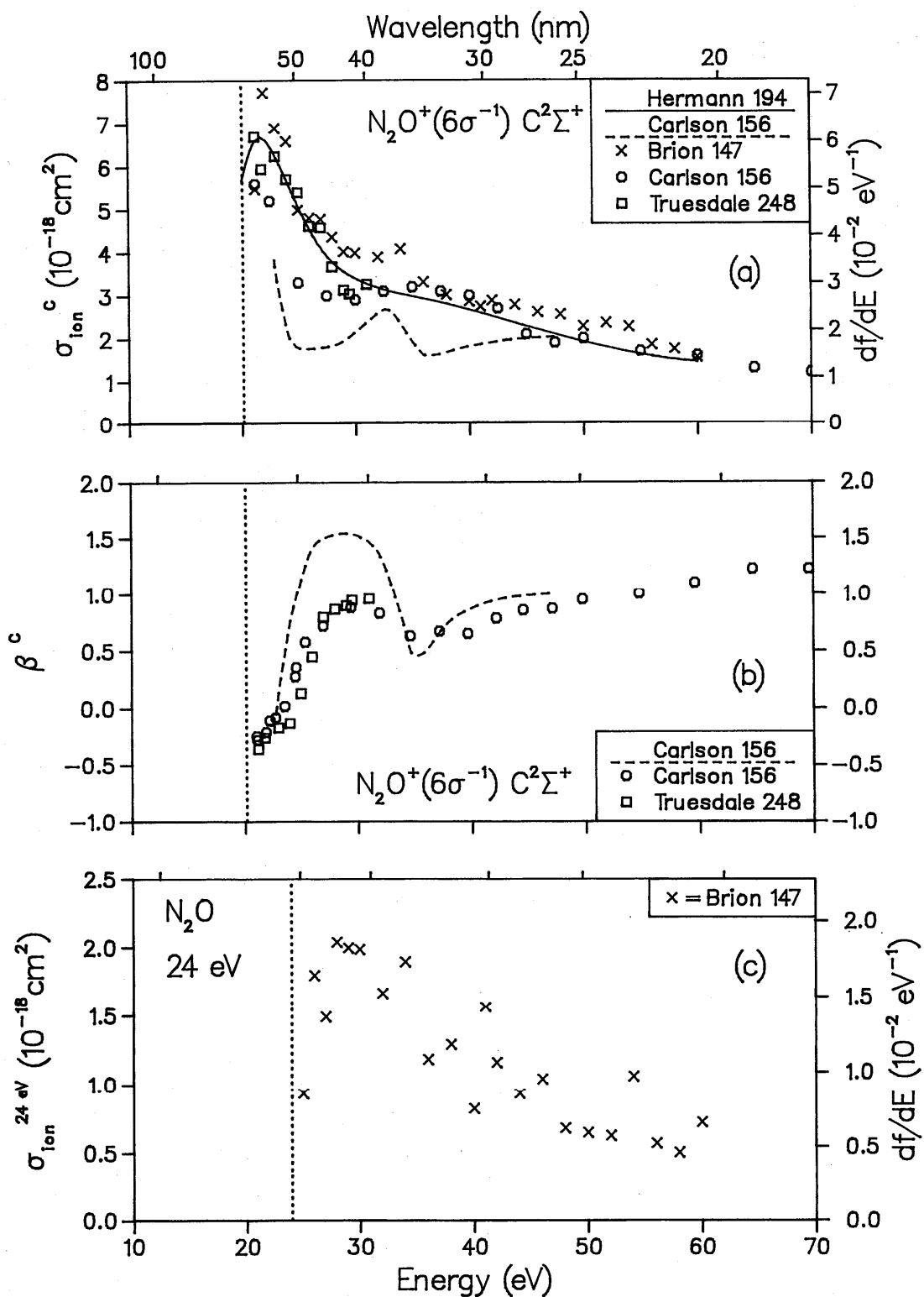
FIG. 46. Partial photoionization cross section for \text{N}_2\text{O} , final ionic state = \text{C}^2\Sigma^+ , (b) photoelectron asymmetry parameter for \text{N}_2\text{O} , final ionic state = \text{C}^2\Sigma^+ , (c) partial photoionization cross section for \text{N}_2\text{O} , final ionic state = PES peak at 24 eV.
