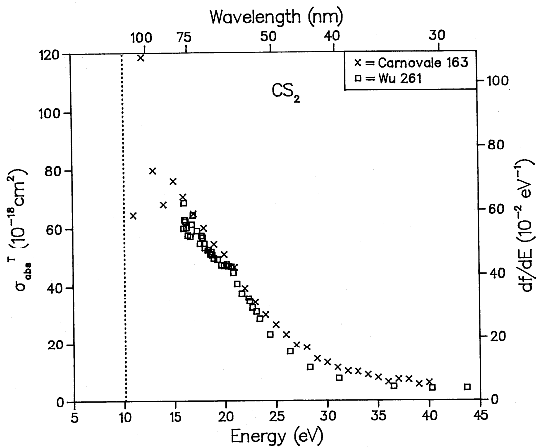
FIG. 80. Total photoabsorption cross section for CS 2 .
