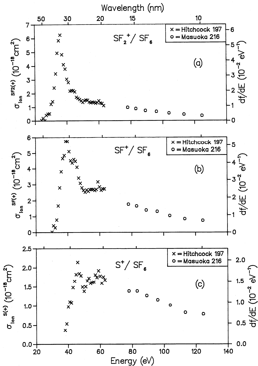
FIG. 101. Partial ionic photoionization cross sections for \text{SF}_6 : (a) product ion = \text{SF}_2^+ , (b) product ion = \text{SF}^+ , (c) product ion = \text{S}^+ .
