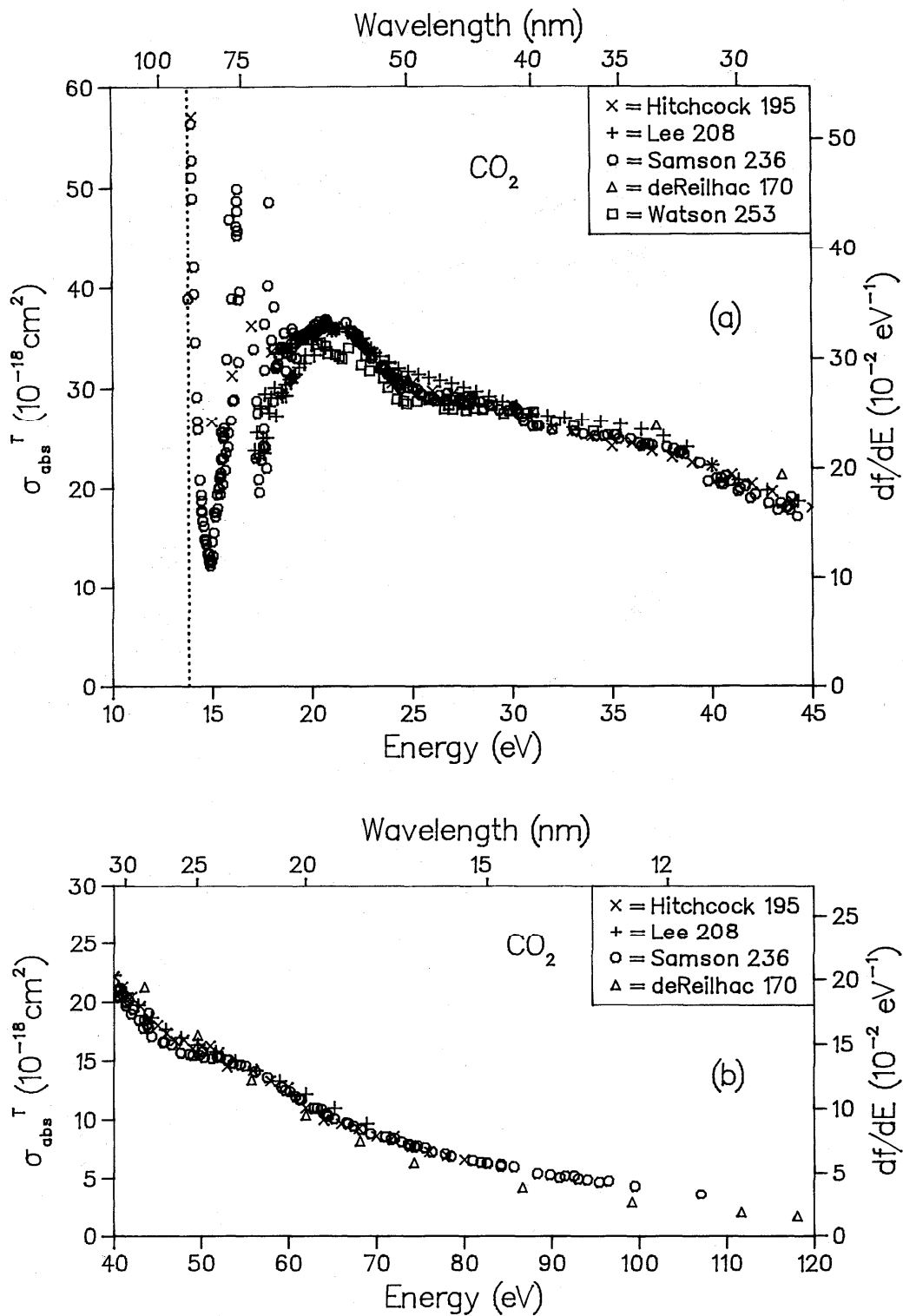
FIG. 37. Total photoabsorption cross section for CO 2 : (a) low-energy range, (b) high-energy range.
