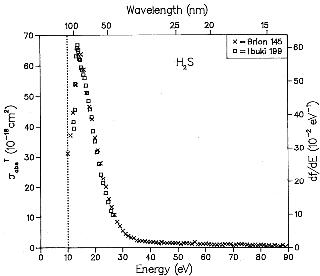
FIG. 75. Total photoabsorption cross section for H 2 S.
