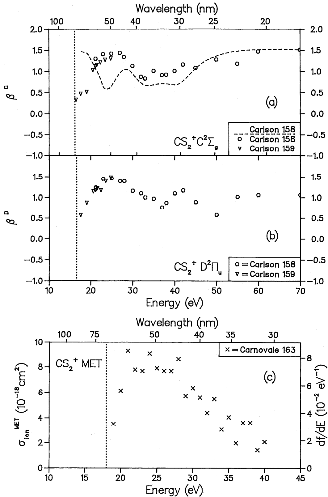
FIG. 84. Photoelectron asymmetry parameters for \text{CS}_2 ; (a) final ionic state = C^2\Sigma_g , (b) final ionic state = D^2\Pi_u , (c) Partial photoionization cross section for \text{CS}_2 , final ionic states = many-body states arising from inner valence ionization.
