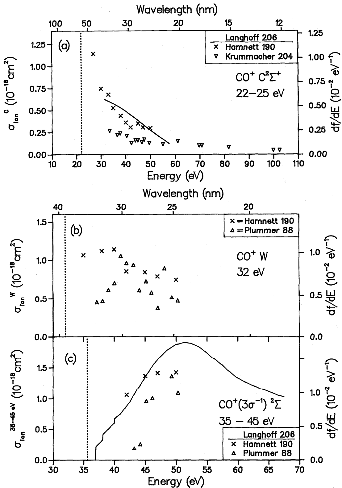
FIG. 27. Partial photoionization cross sections for CO; (a) final ionic state = \text{C}^2\Sigma^+ , (b) final ionic state = W (PES peak at 32 eV), (c) final ionic state = ^2\Sigma (PES peak at 35–45 eV).
