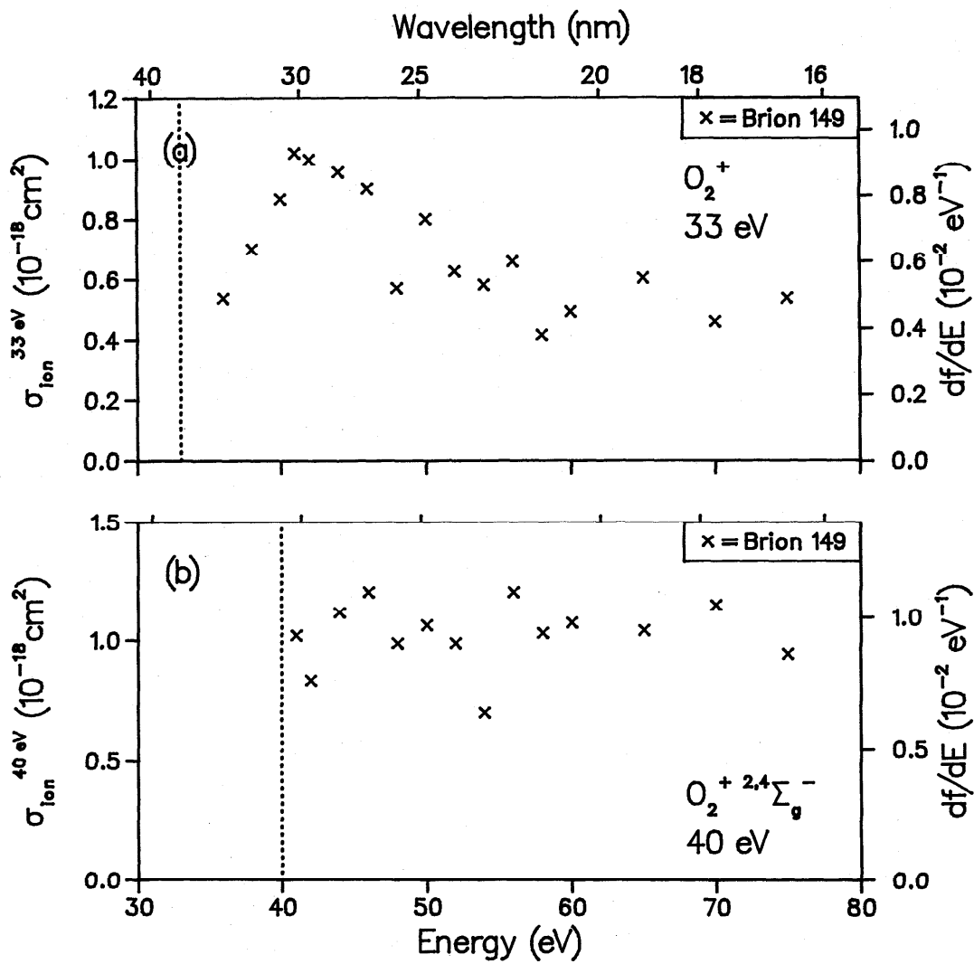
FIG. 22. Partial photoionization cross sections for O 2 ; (a) PES peak at 33 eV, (b) final ionic state = 2,4Σ g - .
