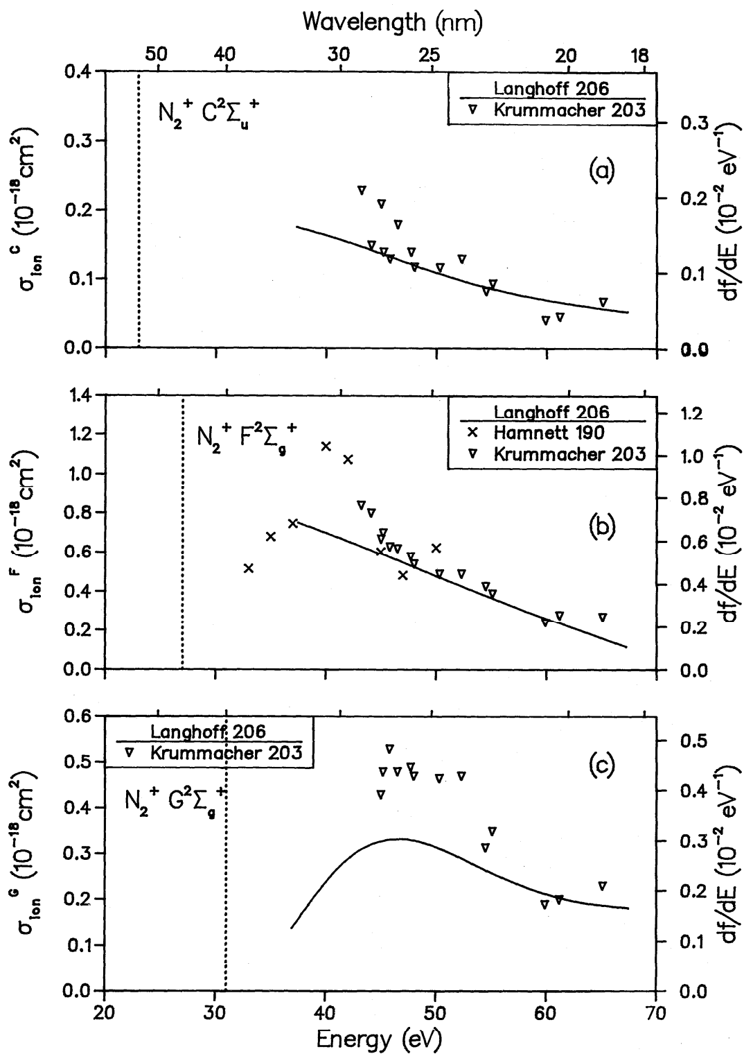
Fig. 16. Partial photoionization cross sections for \text{N}_2 : (a) final ionic state = \text{C}^2\Sigma_u^+ , (b) final ionic state = \text{F}^2\Sigma_g^+ , (c) final ionic state = \text{G}^2\Sigma_g^+ .
