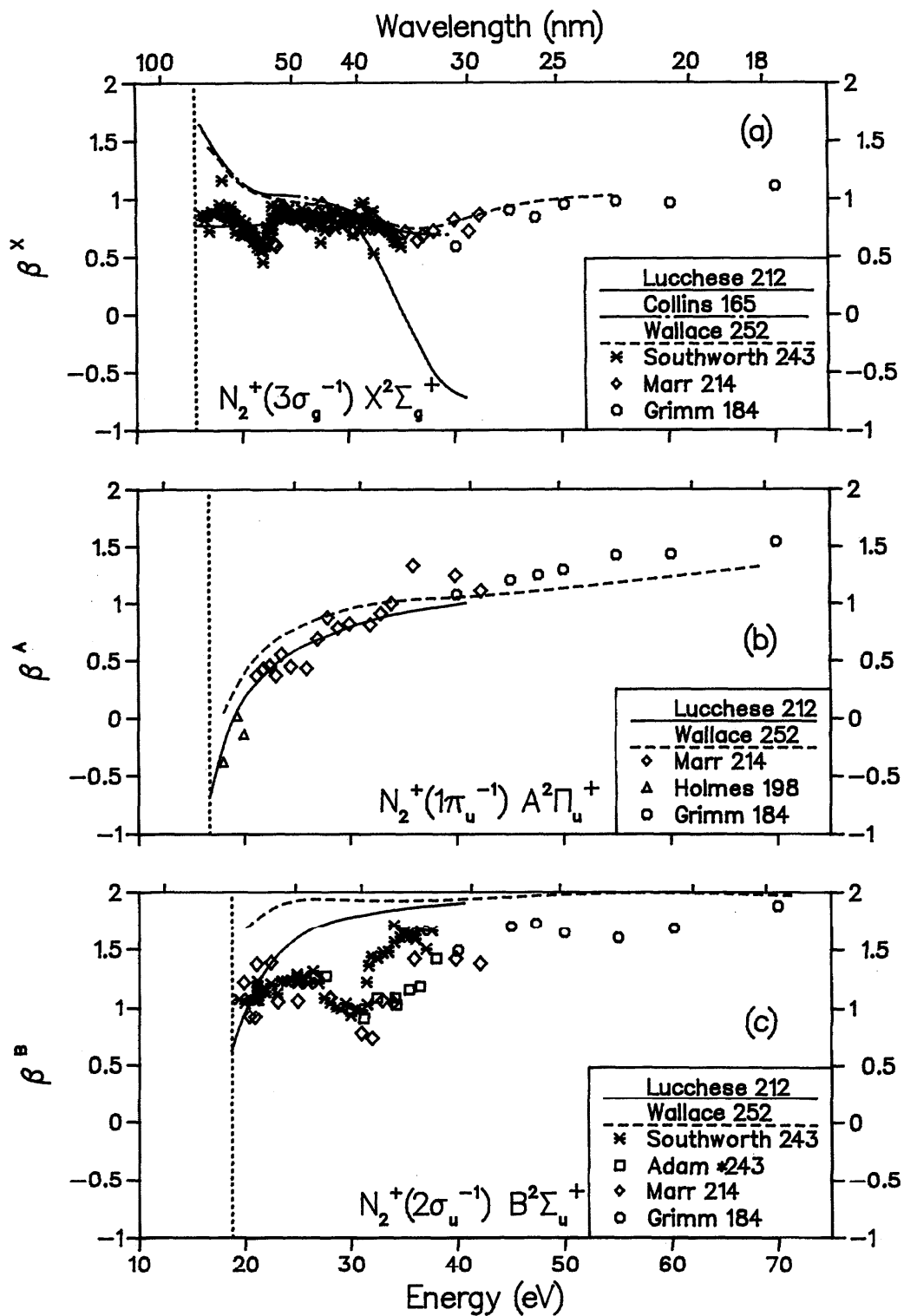
FIG. 15. Photoelectron asymmetry parameters for N_2^+ : (a) final ionic state = X^2\Sigma_g^+ , (b) final ionic state = A^2\Pi_u^+ , (c) final ionic state = B^2\Sigma_u^+ .
