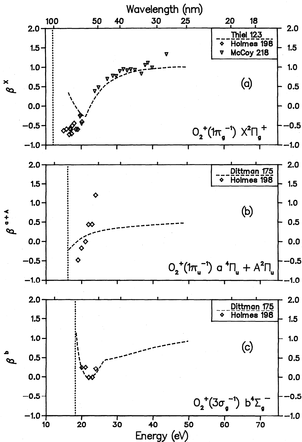
FIG. 20. Photoelectron asymmetry parameters for O_2 ; (a) final ionic state = X^2\Pi_g^+ , (b) final ionic state = a^4\Pi_u + A^2\Pi_u , (c) final ionic state = b^4\Sigma_g^- .
