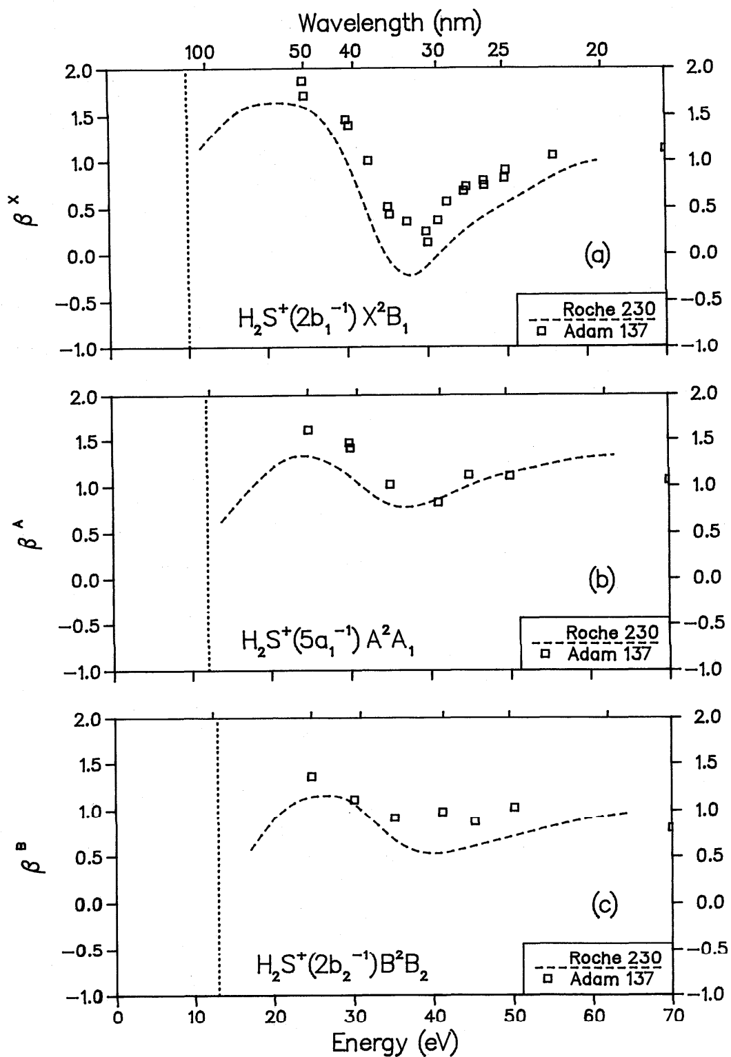
FIG. 77. Photoelectron asymmetry parameters for \text{H}_2\text{S} ; (a) final ionic state = X^2B_1 , (b) final ionic state = A^2A_1 , (c) final ionic state = B^2B_2 .
