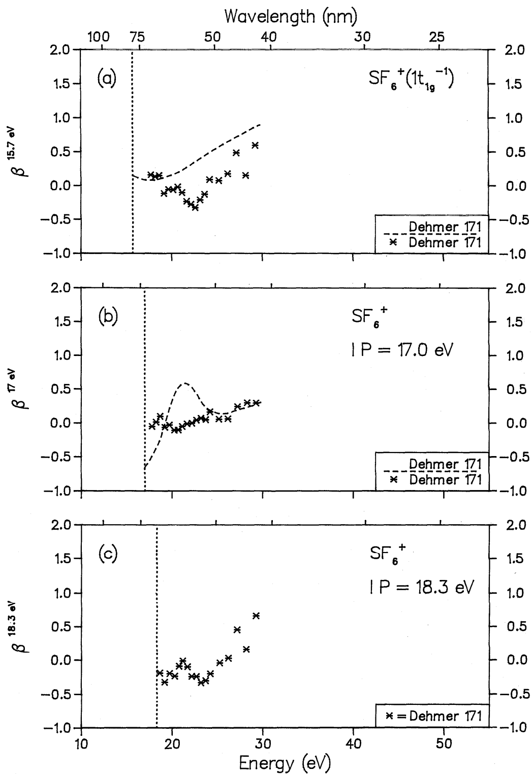
FIG. 98. Photoelectron asymmetry parameters for \text{SF}_6^+ ; PES peak at (a) 15.7 (b) 17.0, and (c) 18.3 eV.
