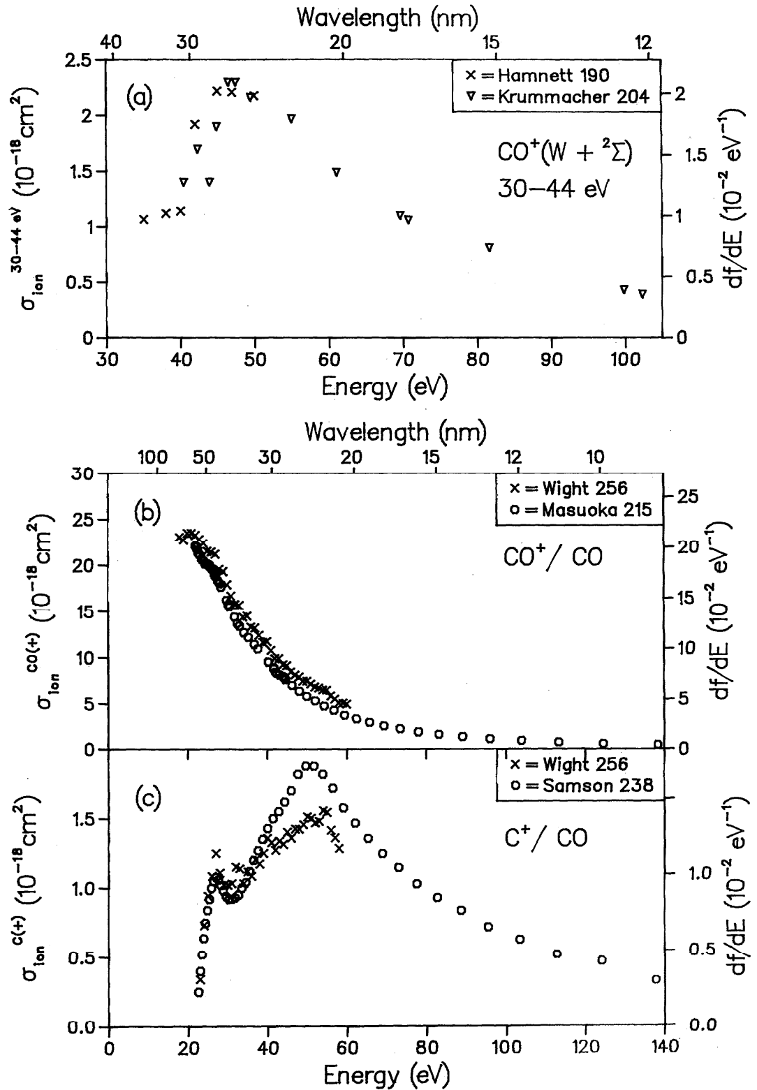
FIG. 28. (a) Partial photoionization cross section for CO, final ionic state = W + {}^2\Sigma (PES peak at 30–44 eV); (b) Partial ionic photofragmentation cross section for CO, product ion = \text{CO}^+ . (c) Partial ionic photofragmentation cross section for CO, product ion = \text{C}^+ .
