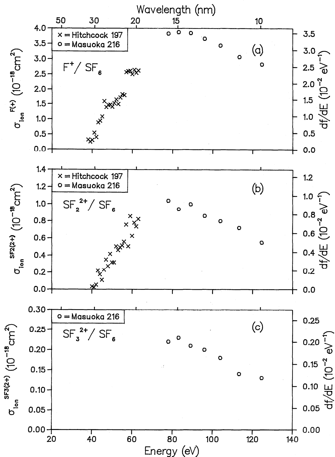
FIG. 102. Partial ionic photofragmentation cross sections for SF 6 ; (a) product ion = F + , (b) product ion = SF 2 2+ , (c) product ion = SF 3 2+ .
