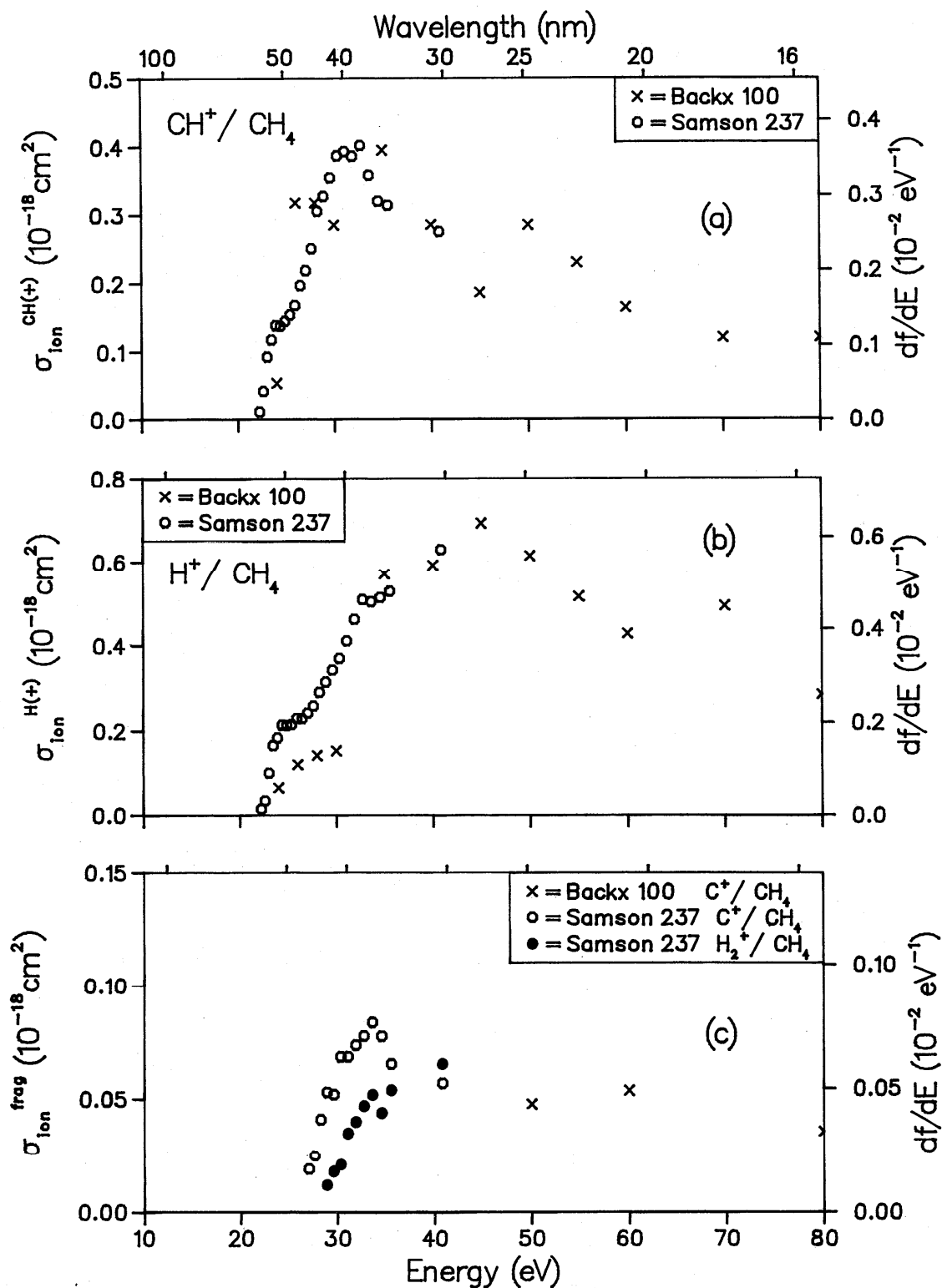
FIG. 63. Partial ionic photofragmentation cross sections for \text{CH}_4 ; (a) product ion = \text{CH}^+ , (b) product ion = \text{H}^+ , (c) product ions = \text{C}^+ and \text{H}_2^+ .
