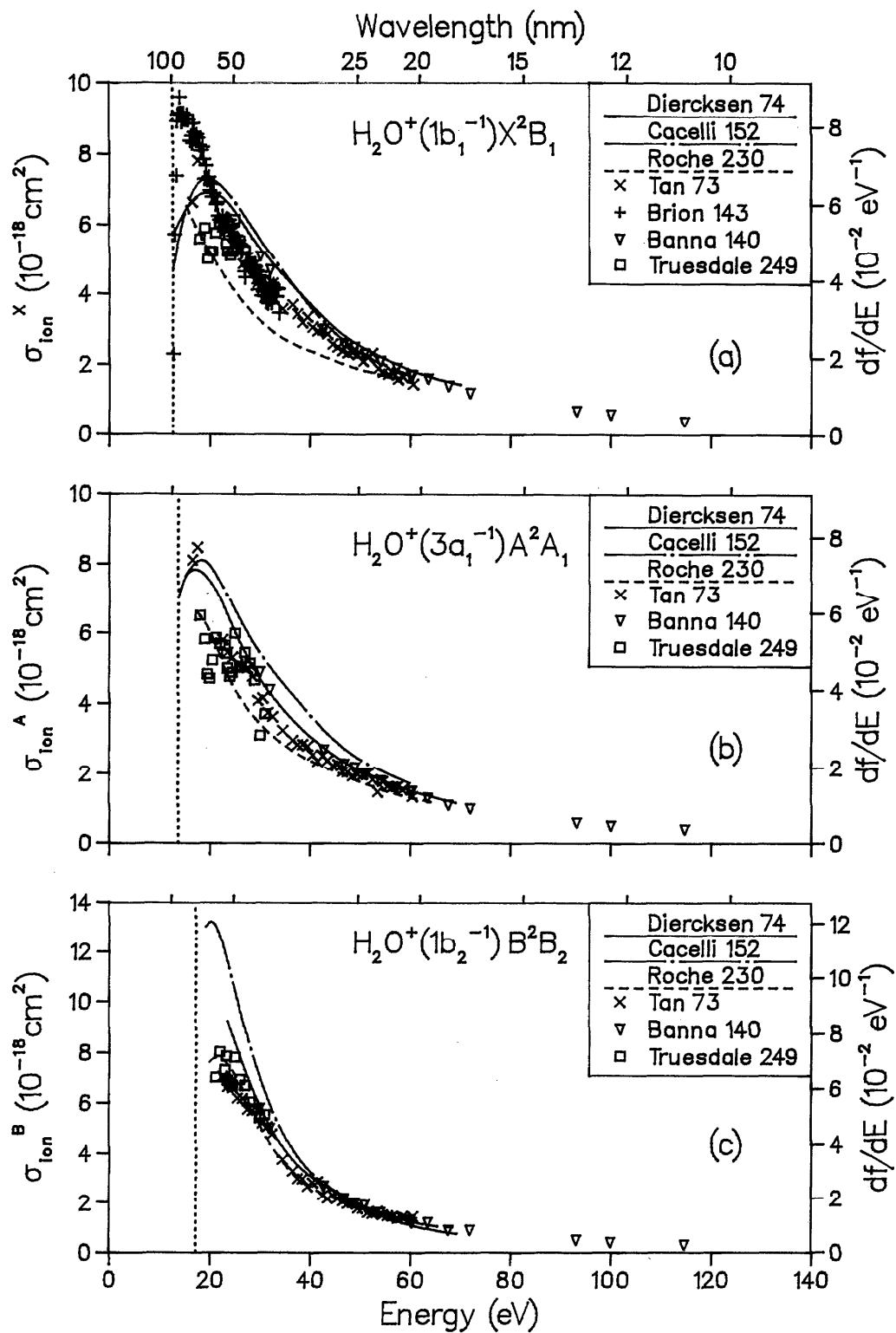
FIG. 50. Partial photoionization cross sections for \text{H}_2\text{O}^+ ; (a) final ionic state = X^2B_1 , (b) final ionic state = A^2A_1 , (c) final ionic state = B^2B_2 .
