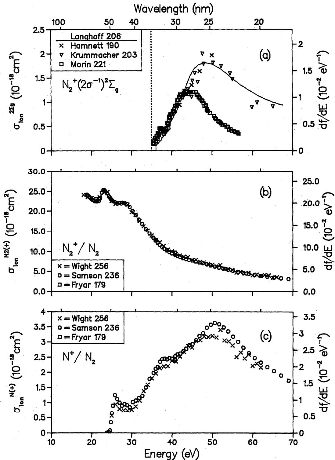
FIG. 17. (a) Partial photoionization cross section for \text{N}_2 ; final ionic state = ^2\Sigma_g . (b) Partial ionic photofragmentation cross section for \text{N}_2 ; product ion = \text{N}_2^+ . (c) Partial ionic photofragmentation cross section, product ion = \text{N}^+ .
