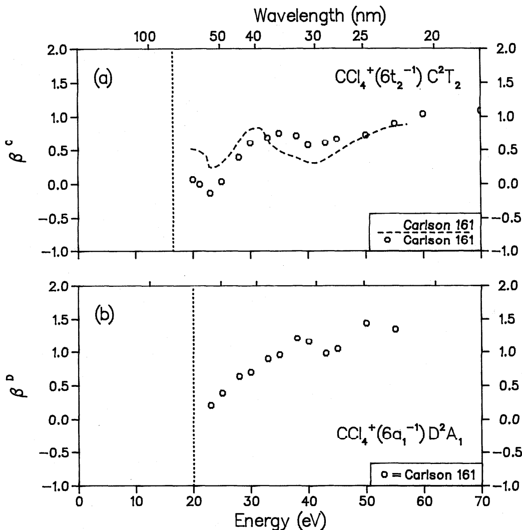
Fig. 111. Photoelectron asymmetry parameters for CCl_4 ; (a) final ionic state = C^2T_2 , (b) final ionic state = D^2A_1 .
