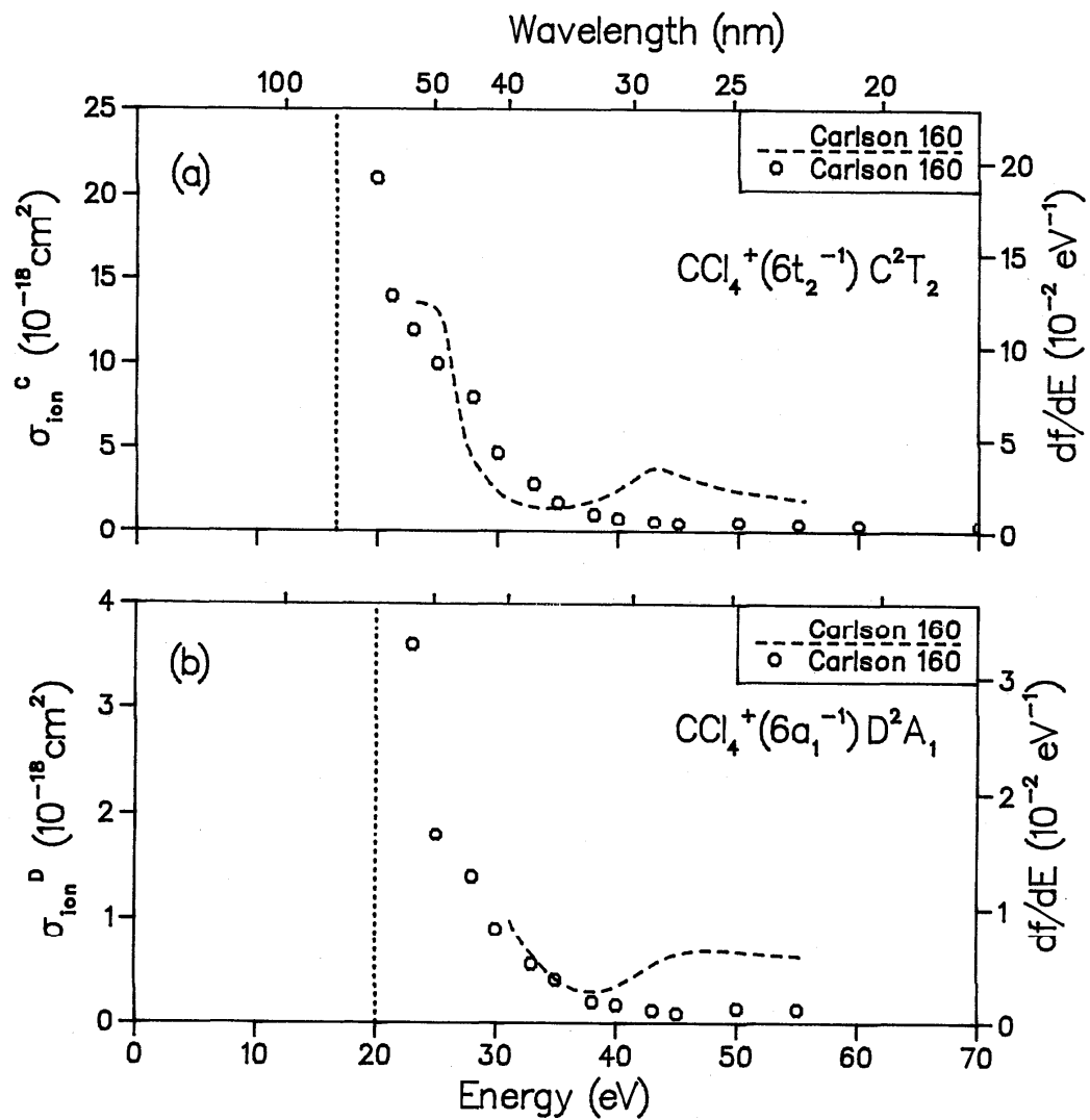
FIG. 110. Partial photoionization cross sections for \text{CCl}_4 ; (a) final ionic state = C^2T_2 , (b) final ionic state = D^2A_1 .
