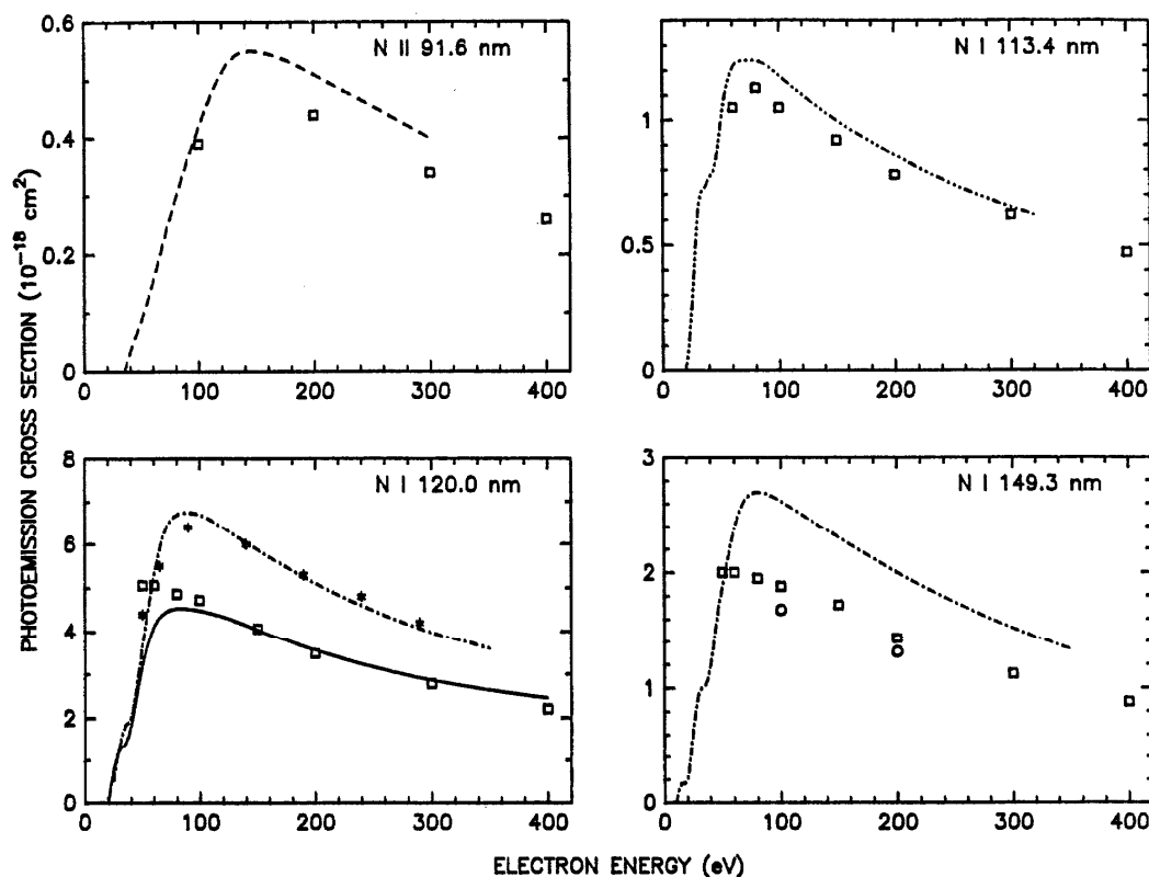
FIG. 4. Comparison of excitation functions for nitrogen transitions. All photoemission cross sections are in 10^{-18} \text{ cm}^2 . Measurements shown are: \square Aarts and de Heer (1971a), - - Mumma and Zipf (1971b), - · - Stone and Zipf (1973), *Huschilt et al. (1981), --- Morgan and Mental (1983), and — and \circ Ajello and Shemansky (1985).
