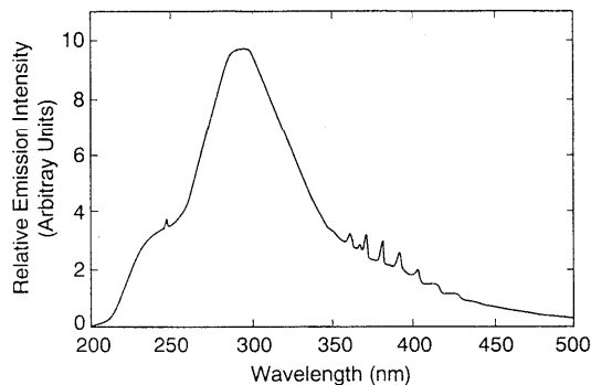
FIG. 28. Optical emission from CF_4 in the wavelength range 200–500 nm produced by collisions of 100 eV electrons with CF_4 (from Refs. 17 and 125).
