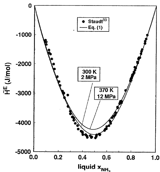
FIG. 14. Molar excess enthalpy \bar{H}^E in the liquid.
