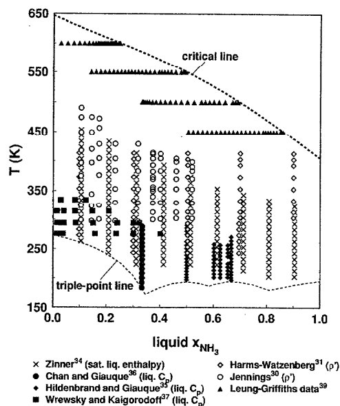
FIG. 3. Distribution of selected saturated liquid densities, enthalpies and isobaric heat capacities.
