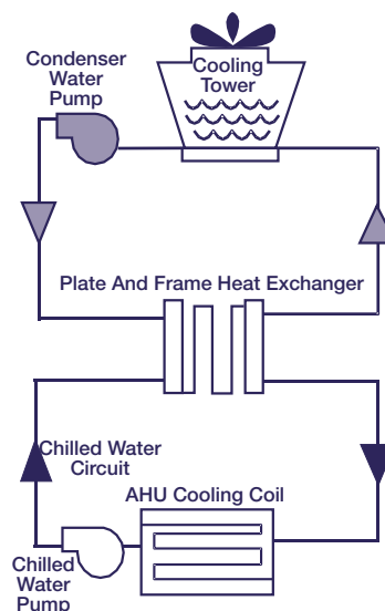
Figure 4: Indirect Water Side Economizer
