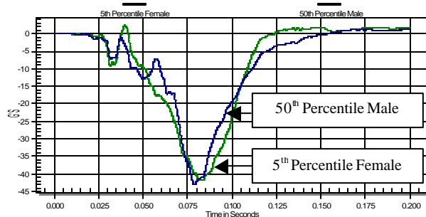
Figure 12: Unbelted passenger chest acceleration results in 48 kmph (30 mph) full frontal rigid barrier crash test of the Ford Econoline (filtered at CFC180).
