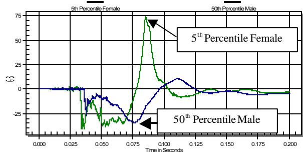
Figure 7: Head acceleration trace of the 5 th percentile female passenger dummy's head hyperextended rearward and the comparable response from the 50 th percentile male dummy (filtered at CFC1000).
