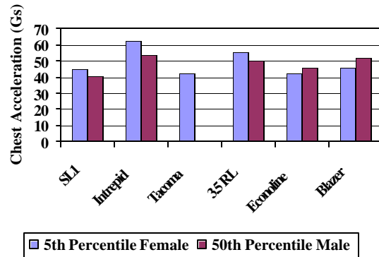
Figure 10: Unbelted passenger chest acceleration results for the six pairs of 48 kmph (30 mph) full frontal rigid barrier crash tests.
