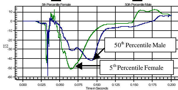
Figure 1: Passenger head acceleration signals with evidence of early head-to-air bag contact in the Toyota Camry tests (filtered at CFC1000).
