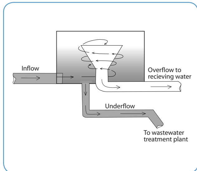
Figure 1. Simplified diagram of a vortex separator.
