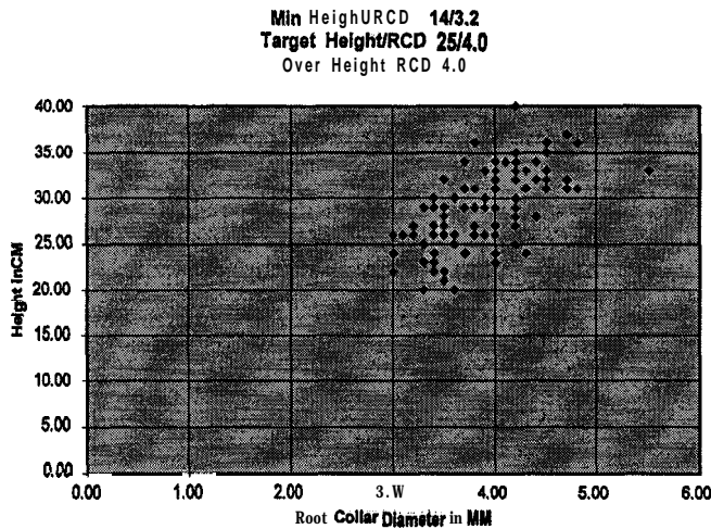
Figure 6—Scattergram Interior Spruce PSB415D.
