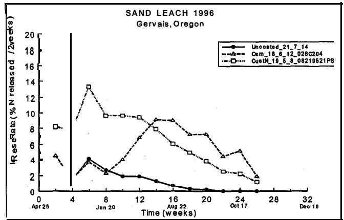
Figure 1-Release curves.
