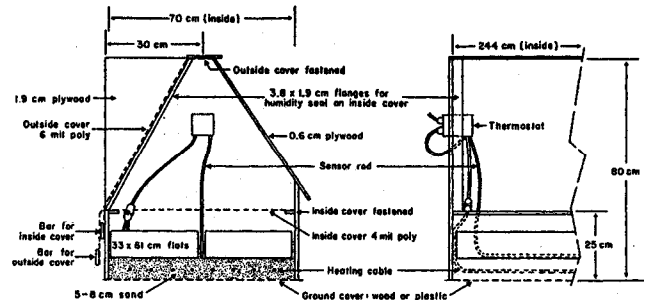
Diagram of outside propagation frames
