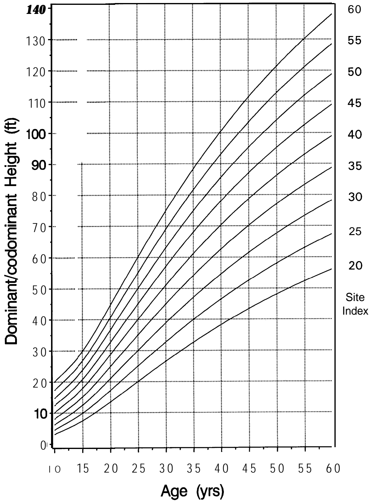
Figure 2-White pine polymorphic site index curves based on Frothingham's data, base age 25
