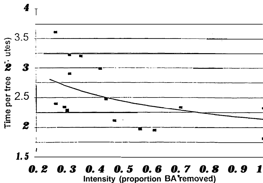
Figure 2. — Predicted average felling time per tree within a stand.
