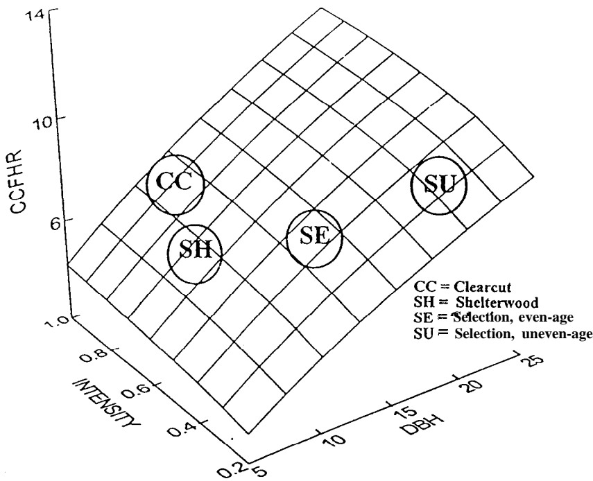
Figure 3. — Felling productivity by harvest intensity and stem diameter.
