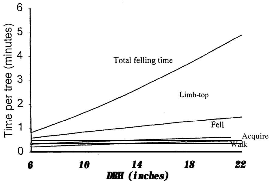
Figure 1.— Predicted felling time by operation per tree based on DBH
