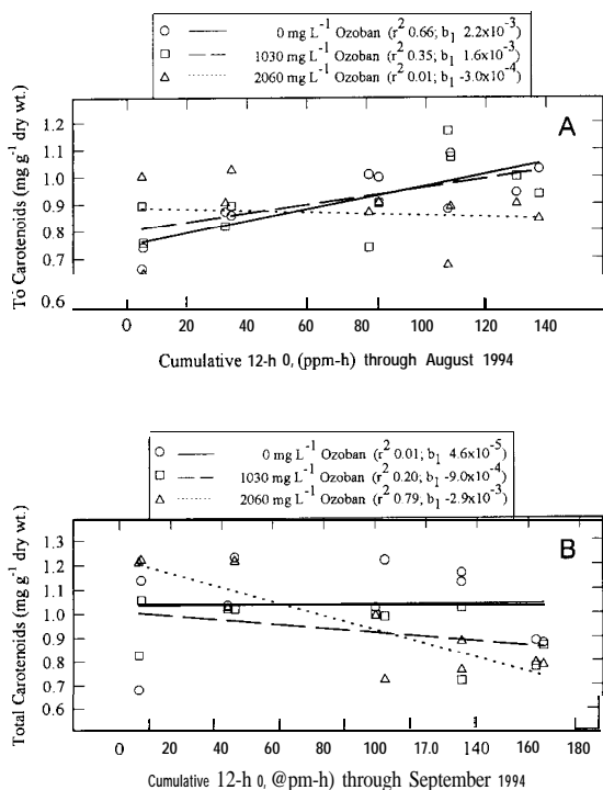
Fig. 5. Linear regression analysis for total carotenoids on cumulative ozone in August (A) and September (B) for Ozoban-treated S6PT2 loblolly pine seedlings. Seedlings treated with 2060 mg liter -1 Ozoban had a significantly more negative slope than either 0 or 1030 mg liter -1 Ozoban.
