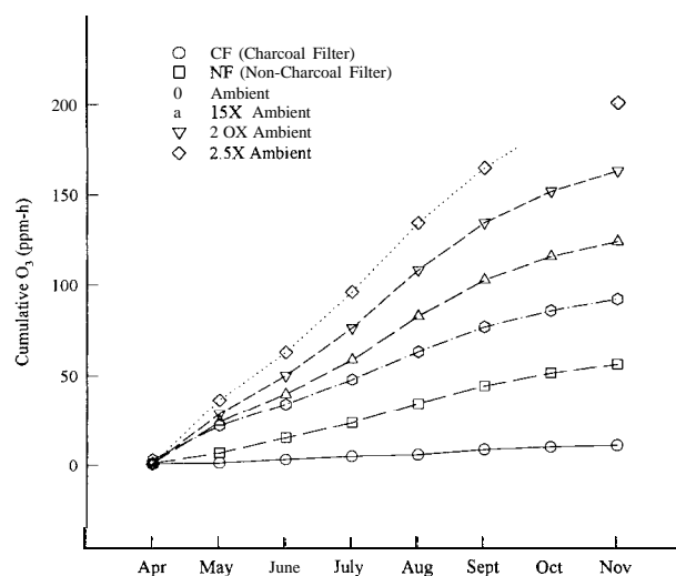
Fig. 1. Cumulative 12-h ozone for each exposure level from 25 April to 19 November 1994 in east Texas.
