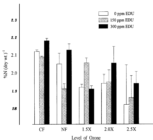
Fig. 6. Concentration of total foliar N (+ 1 SD) in dried tissue of ethylenediurea (EDU)-treated S6PT2 loblolly pine seedlings for each EDU treatment level by ozone exposure in October 1994. Significant ozone by EDU-concentration interaction was observed. N concentration was greatest for seedlings treated with 300 ppm EDU at all ozone levels except 1.5x
