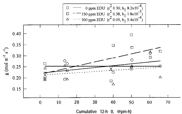
Fig. 4. Linear regression analysis for g on cumulative ozone for EDU-treated S6PT2 loblolly pine seedlings in June 1994. Seedlings treated with 150 ppm EDU exhibited a significantly greater slope compared to the combined slope.
