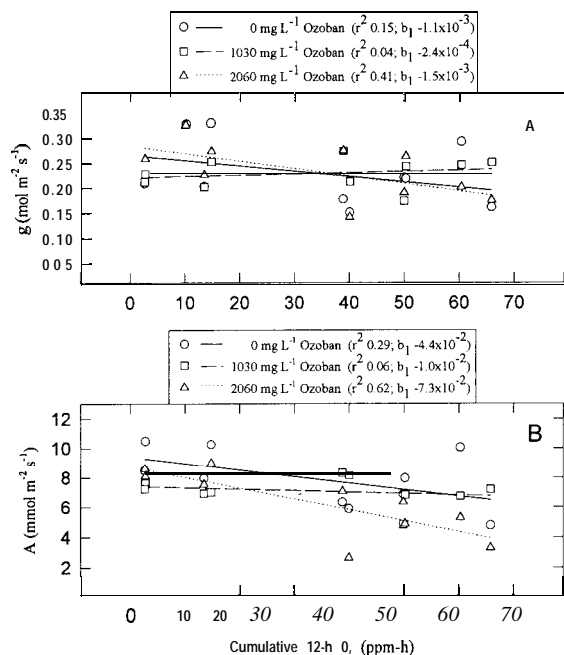
Fig. 2. Linear regression analysis for g (A) and A (B) on cumulative ozone for Ozoban-treated S6PT2 loblolly pine seedlings in June 1994. The rate of stomatal conductance and photosynthesis for seedlings treated with 1030 mg liter -1 Ozoban did not decrease substantially with increasing ozone compared to that of the combined data.
