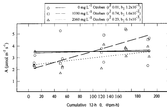
Fig. 3. Linear regression analysis for A on cumulative ozone for Ozoban-treated S6PT2 loblolly pine seedlings in October 1994. Seedlings treated with 1030 mg liter -1 Ozoban exhibited a greater slope than seedlings treated with 0 or 2060 mg liter -1 Ozoban.
