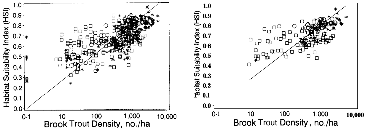
Fig. 3. Habitat suitability index (HSI = 100 \times predicted standing stock / maximum standing stock) versus measured standing stock in streams of the southern Blue Ridge Province. Diagonal lines represent perfect agreement between HSI and measured standing stock; circles = surveys by Fowler (1985); squares = surveys by the North Carolina Wildlife Resources Commission; asterisks = surveys by the U.S. National Park Service (Parker MS). Upper panel: all streams ( n = 250 ); lower panel: brook trout ( Salvelinus fontinalis ) streams, no rainbow trout ( Oncorhynchus mykiss ) present ( n = 172 ).
