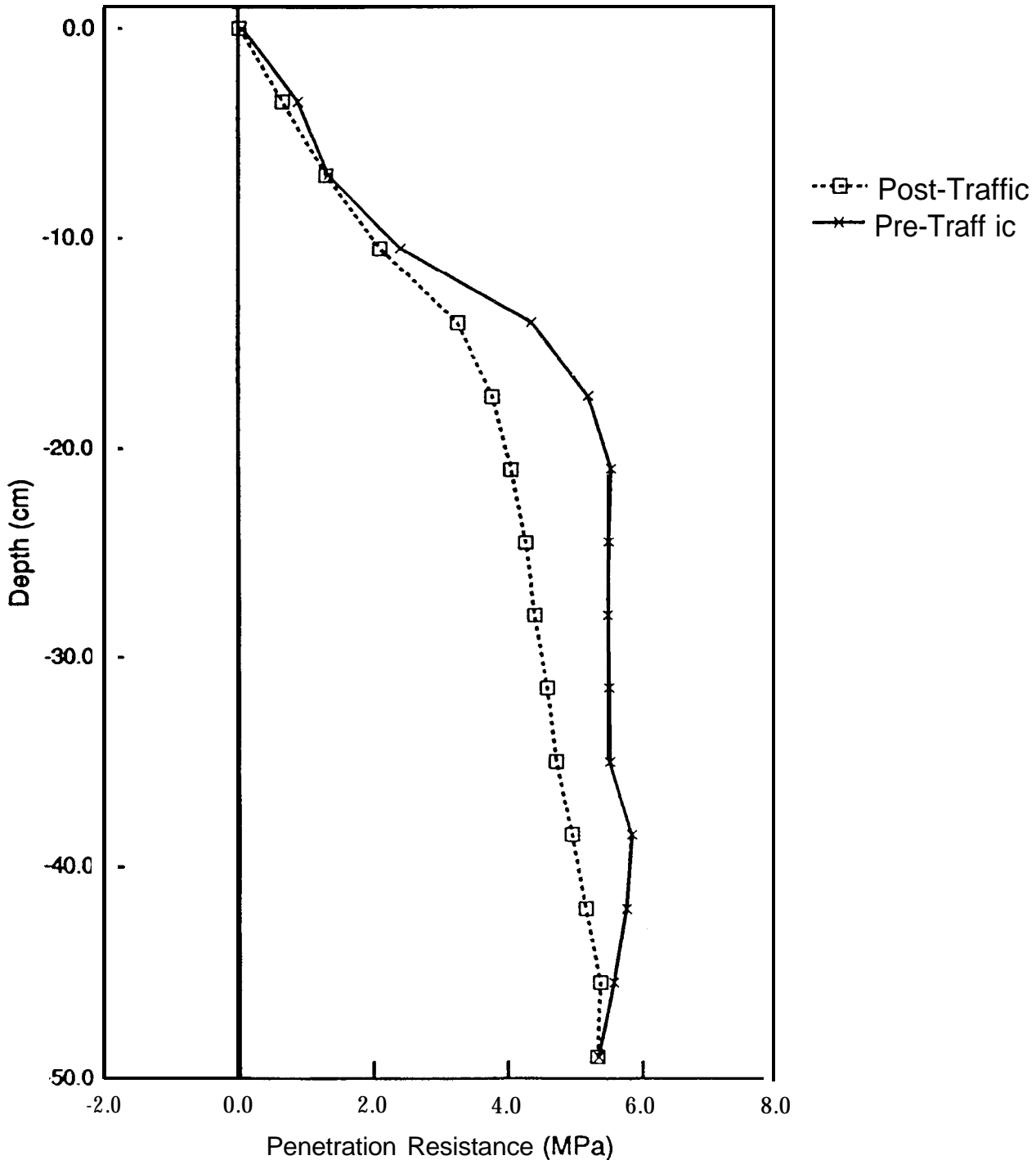
Figure 1. Soil strength, bare plots, dry condition, 1 pass.
