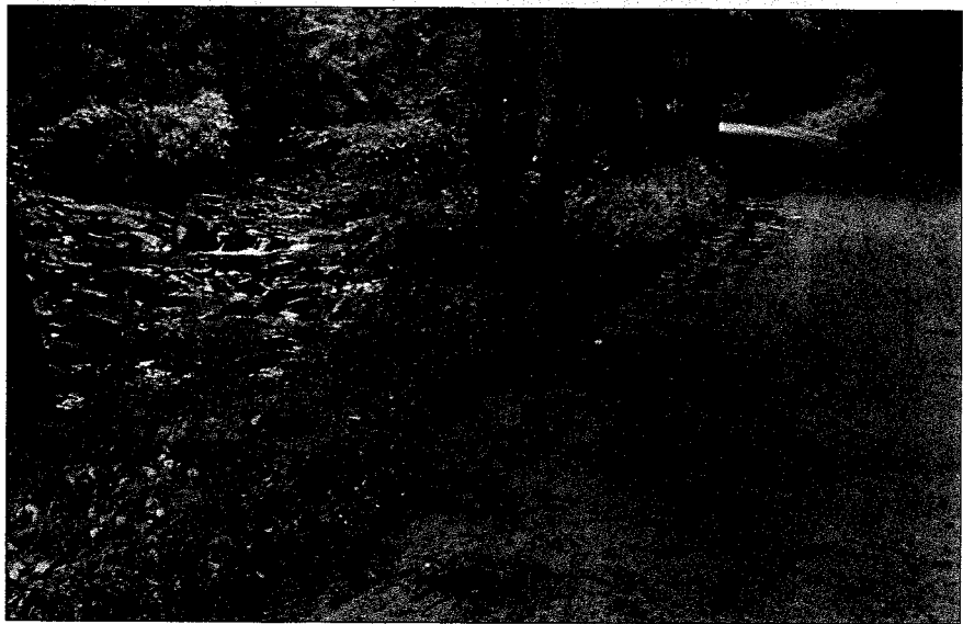
This long-established road is too close to a stream, and sediment flowed from the roadbed into the channel during storms. The roadside berm was constructed of gravel during regrading and now prevents storm runoff from entering Curtis Creek. Runoff and sediment flow along the road's edge to a disposal site away from the stream.
