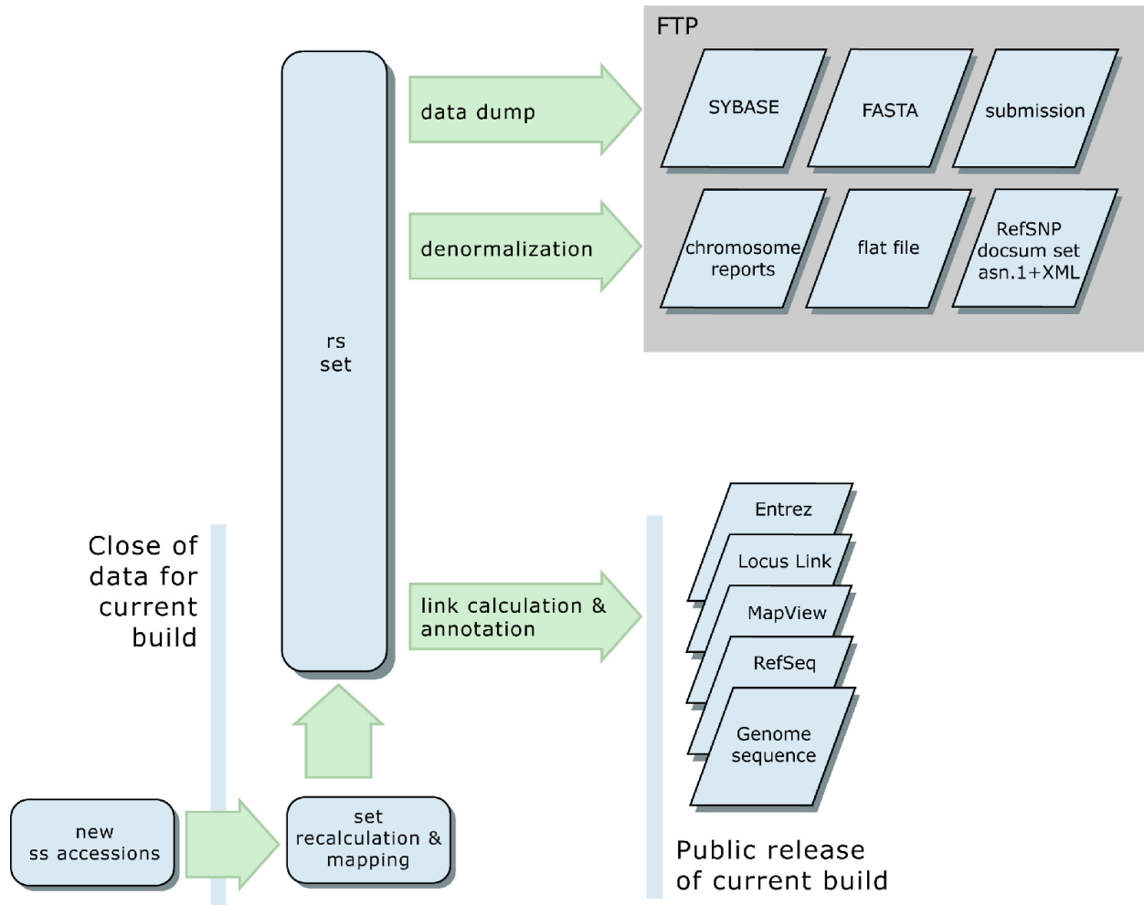
Figure 4: The dbSNP build cycle. The dbSNP build cycle starts with close of data for new submissions. We map all data, including existing refSNP clusters and new submissions, to reference genome sequence if available for the organism. Otherwise, we map them to non-redundant DNA sequences from GenBank. We then use map data on co-occurrence of hit locations to either merge submissions into existing clusters or to create new clusters. We then annotate the new non-redundant refSNP (rs) set on reference sequences and dump the contents of dbSNP in a variety of comprehensive and denormalized formats on the dbSNP FTP site for release with the online build of the database.
