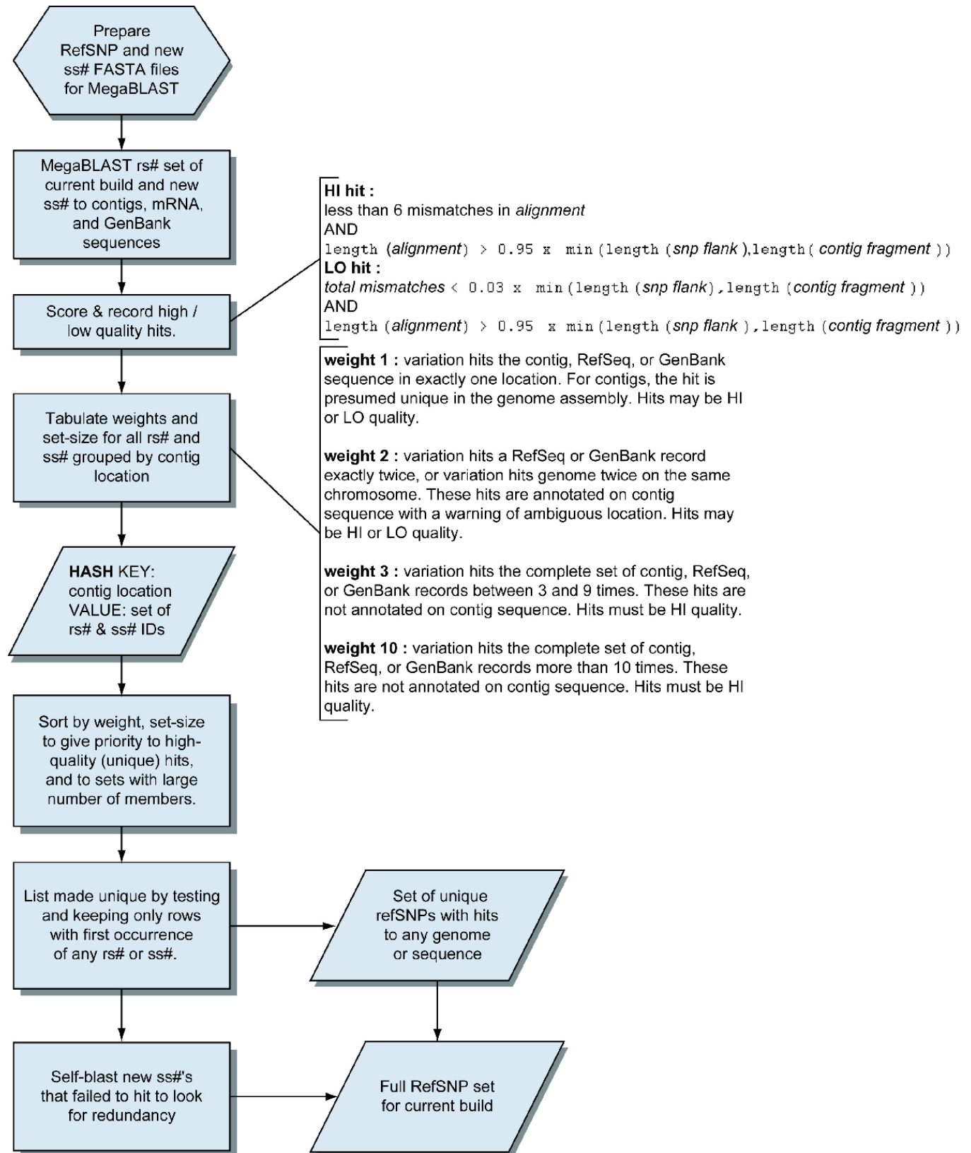
Figure 6: The dbSNP reclustering process. We define clusters on shared locations (refSNPs) when we BLAST all existing refSNPs against contig sequence. In cases where contig sequence is not available or the variation is defined in a mRNA flanking sequence that will not map to a contig, we compute the refSNP set based on hits to the RefSeq or GenBank sequences for the organism. We rank map
