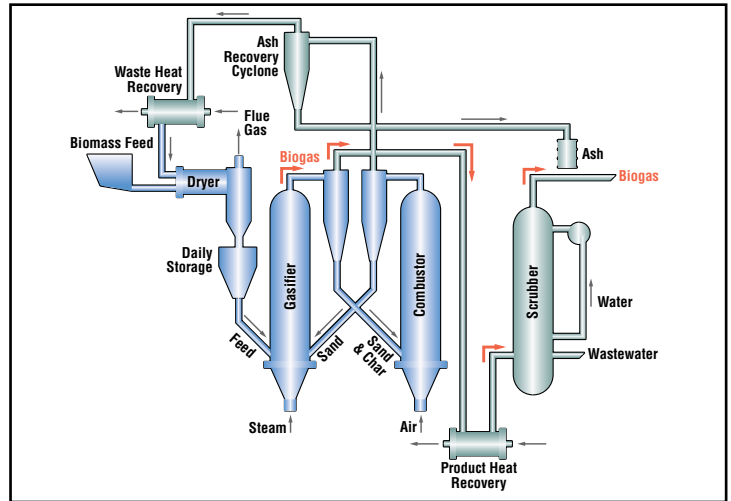
Vermont gasifier schematic
