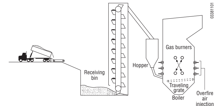
Figure 2. Schematic of a typical traveling-grate spreader-stoker.
