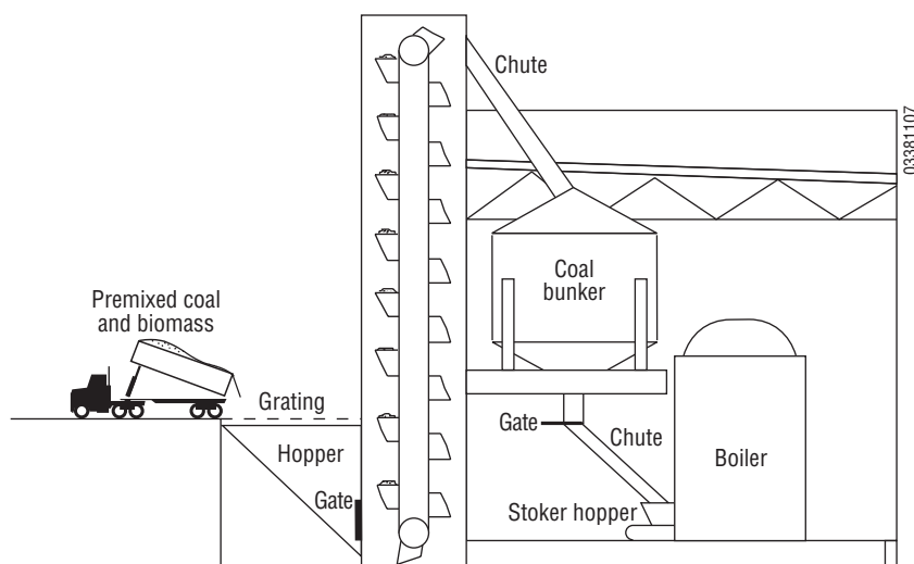
Figure 8. A typical stoker boiler conveyor system receiving premixed coal and biomass (Adapted from J. Cobb et al., June 1999).
