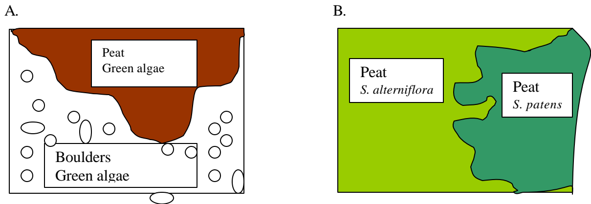
Figure 8. (A) The assemblage “Green Algae” growing on two different substrates. Two distinct polygons were mapped. (B) Two different assemblages growing on Peat substrate. Two distinct polygons were mapped.
