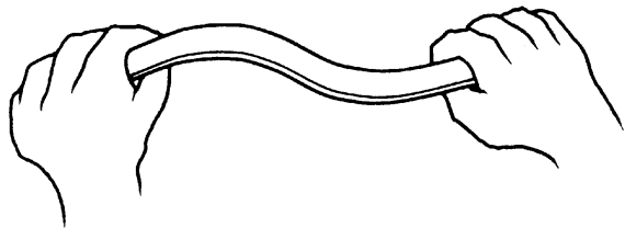
Buildup of potential energy in bent stick and deformed rocks
