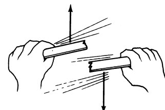
Breaking stick produces energy release
