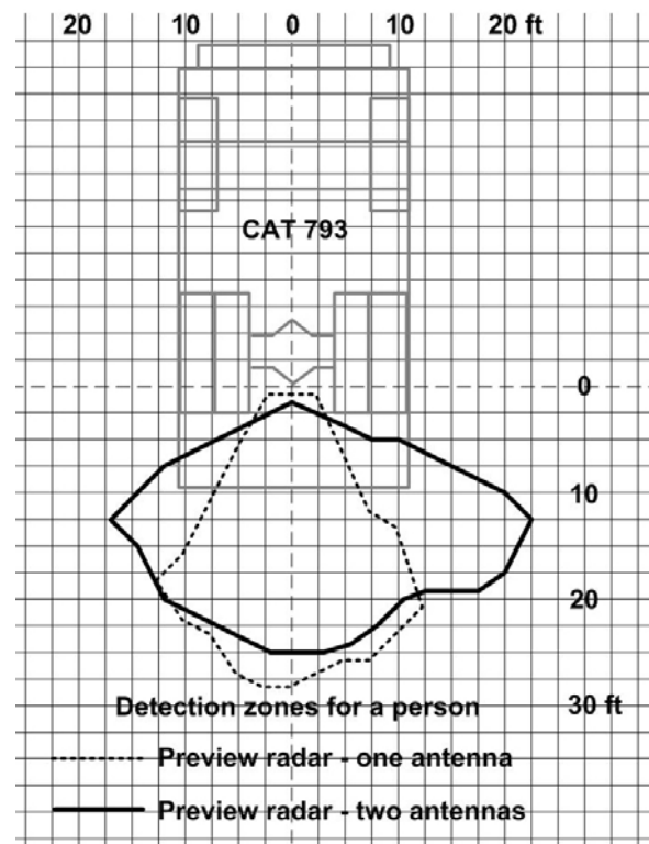
Figure 2. Comparison of detection zones for single- and dual-antenna Preview radar system.
