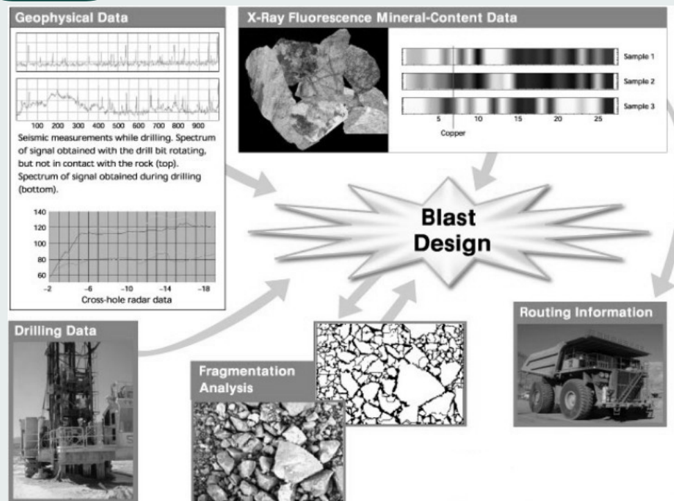
Flow diagram showing the data inputs into blast design.
