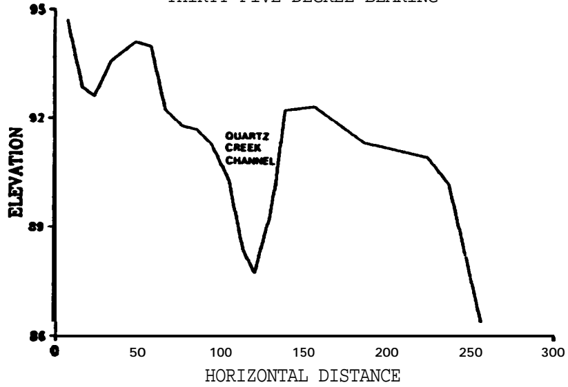
Appendix A12. A cross-sectional view of the Quartz Creek delta along the 35^{\circ} bearing, from the plumb bob point to the bench mark #241.
