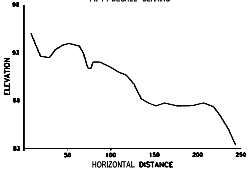
Appendix A13. A cross-sectional view of the Quartz Creek delta along the 50^{\circ} bearing, from the plumb bob point to the bench mark #241.
