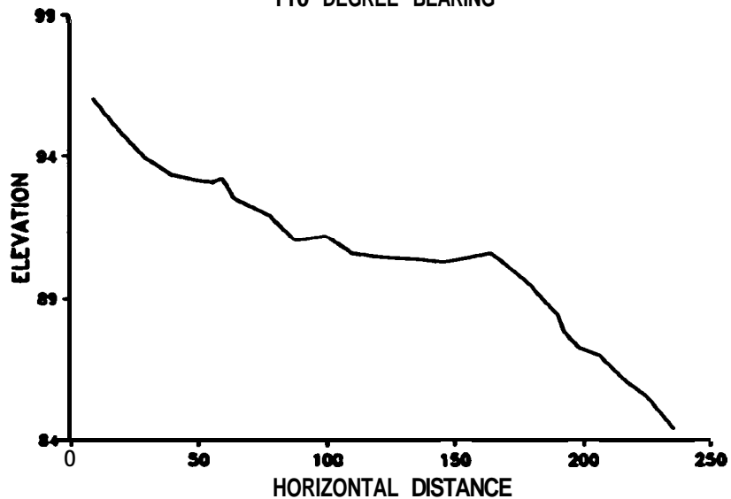
Appendix A17. A cross-sectional view of the Quartz Creek delta along the 110° bearing, from the plumb bob point to the bench mark #241.
