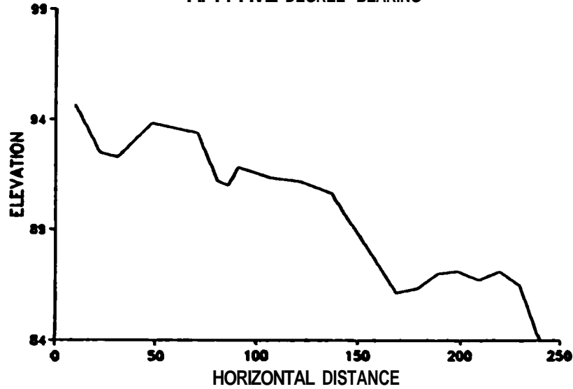
Appendix A14. A cross-sectional view of the Quartz Creek delta along the 55^\circ bearing, from the plumb bob point to the bench mark 5241.
