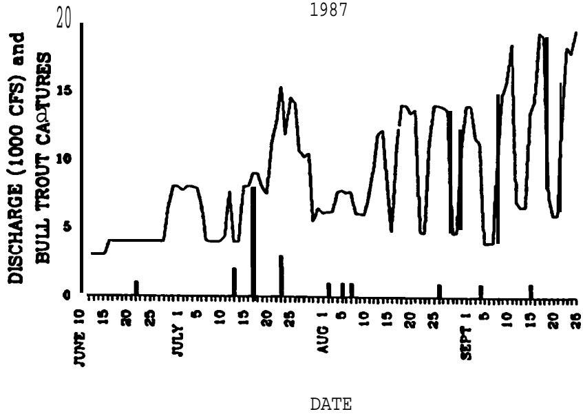
Figure 44. Timing of bull trout entry into Quartz Creek, 1987.
