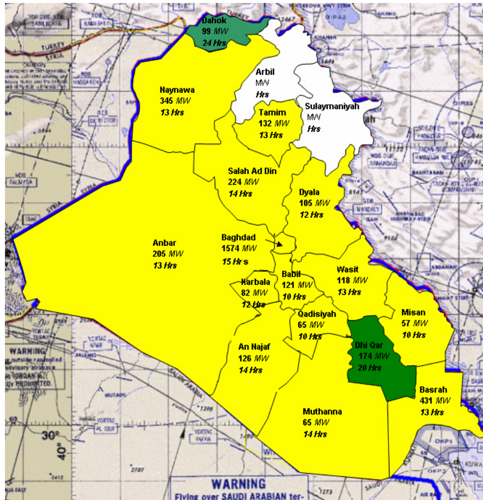
Average Electrical Power Distribution per Governorate as of 18 August 2004
