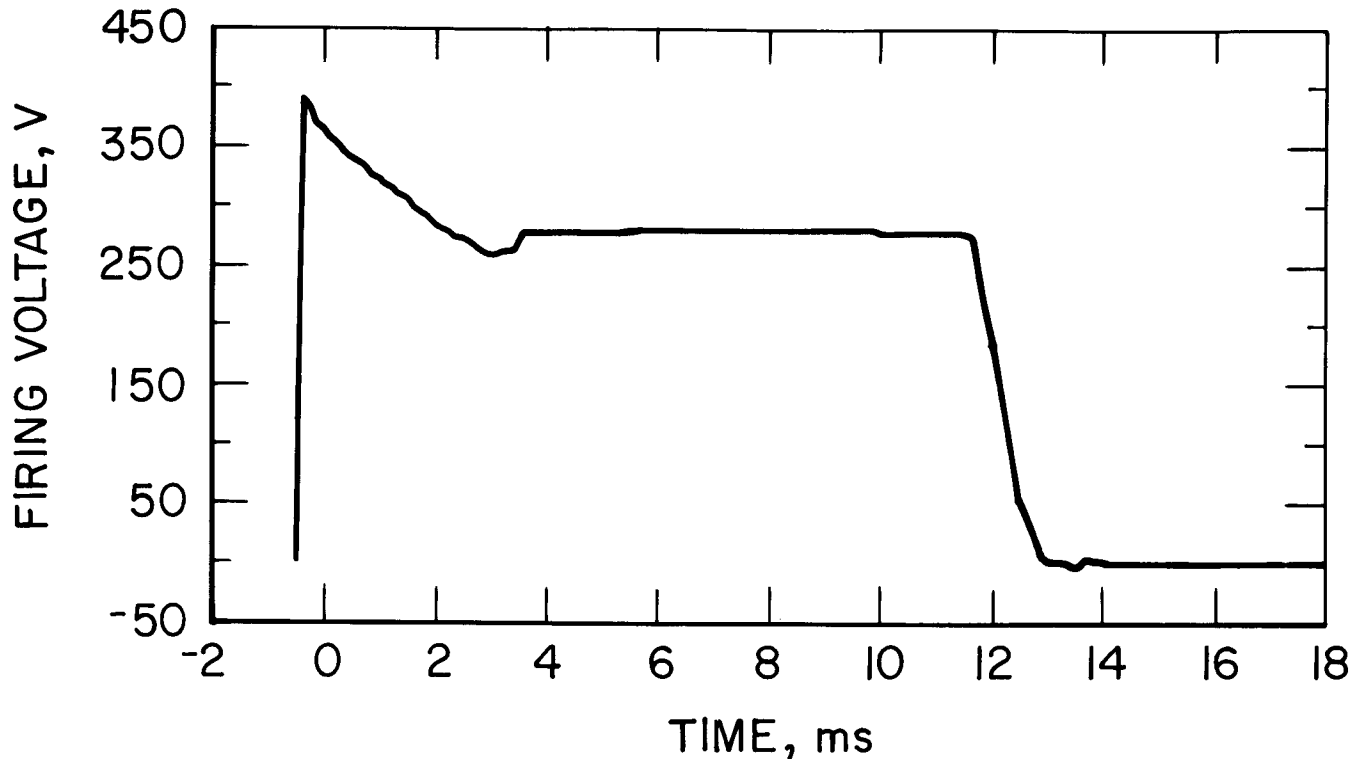
FIGURE 3. - Typical firing voltage signature.
