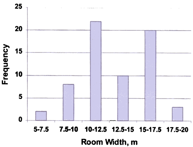
FIG. 4 Histogram of room widths for 65 underground stone mines.
