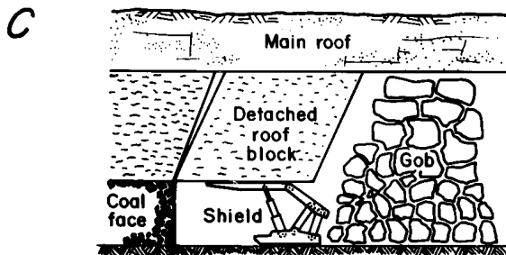
Figure 23.—Four general categories of strata behavior pertaining to shield loading. A, Main roof convergence; B, periodic weighting; C, detached immediate roof; D, deflection of immediate roof.
