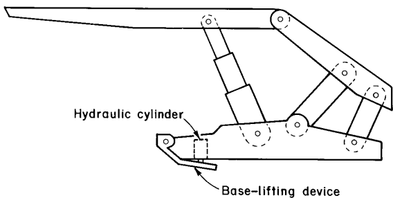
Figure 9.—Base-lifting device.
