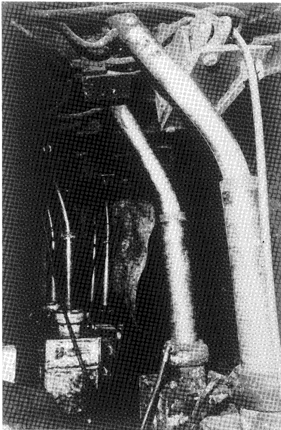
Figure 1.—Bending of leg cylinders in chock support.
