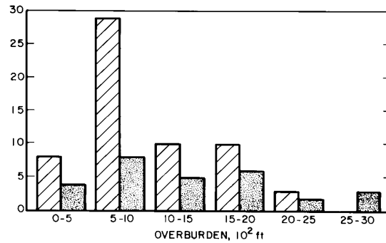
Figure 22.—Selection of two-leg and four-leg shields as function of seam height, panel width, and depth of cover.
