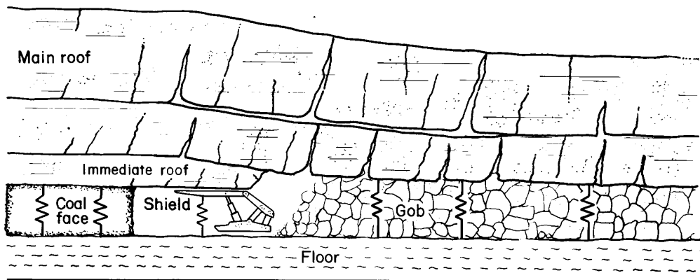
Figure 13.—Mechanics of roof behavior and manifestation of shield loading.
