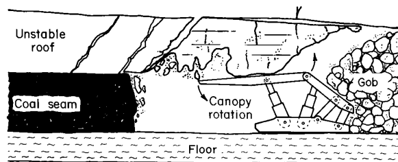
Figure 19.—Four-leg shield operation in cavity-prone conditions illustrating problems of canopy control.
