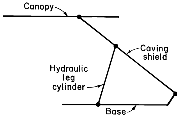
Figure 2.—Horizontal stiffness provided in early shield design by mechanically connecting canopy with base.
