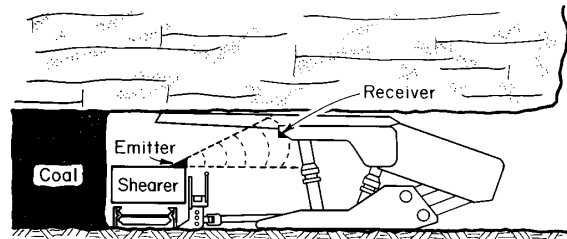
Figure 10.—Shearer-initiated electrohydraulic shield control system.
