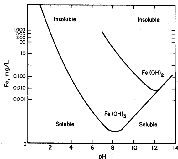
Figure 1.—Solubility curves for ferrous and ferric iron. [Source: U.S. Environmental Protection Agency (1)]
