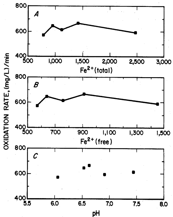
Figure 3.—Oxidation rate. A, Versus \text{Fe}^{2+} (total); B, versus \text{Fe}^{2+} (free); C, versus pH.
