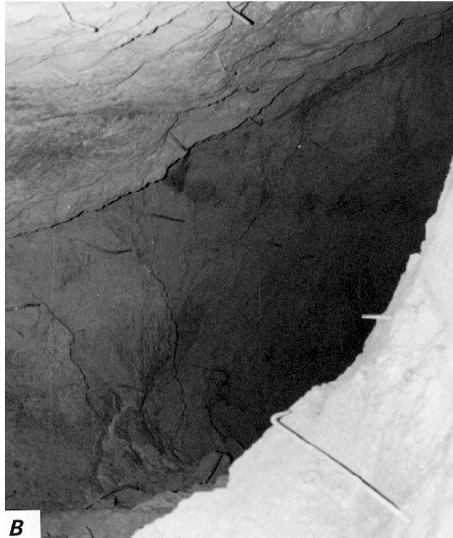
Breakouts observed in Silver shaft ore passes on 5100 level. A, Plan view. Circle (dotted line) indicates original shape of ore pass, while ellipse (solid line) indicates final shape after breakouts occurred. B, Breakout as observed looking down north ore pass.
