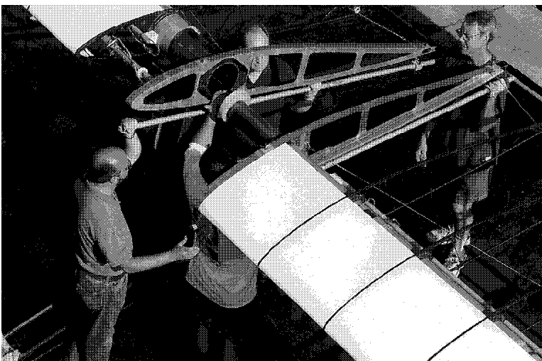
Assembly of the Centurion structure at AeroVironment's Simi Valley Design and Development Center
